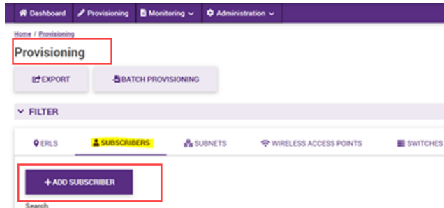
Figure 5 : Add Subscriber
