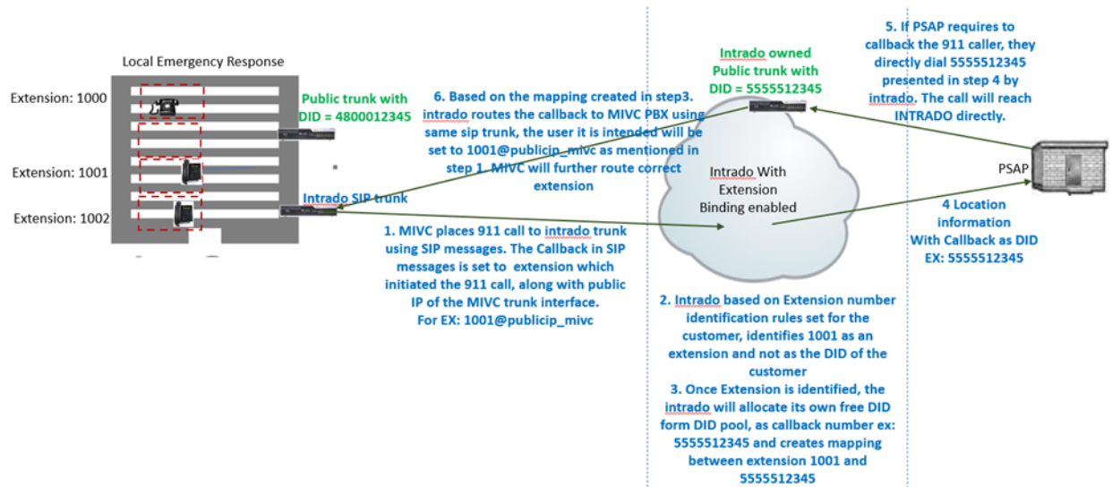
Figure 11 : Intrado Extension Bind Flow
