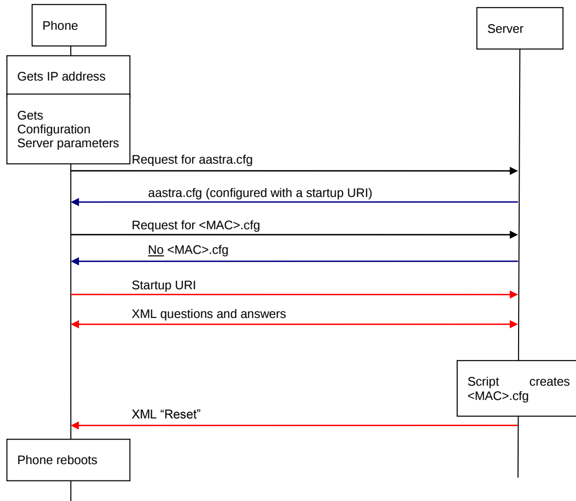
Figure 93: Auto-configuration message flow
