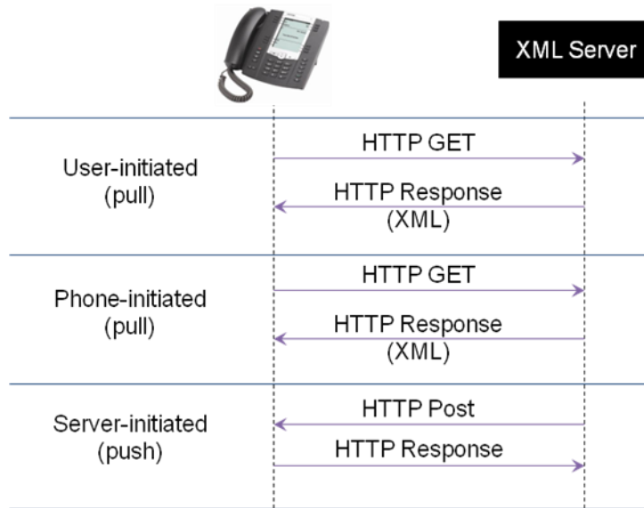
Figure 92: HTTP flow for XML applications
