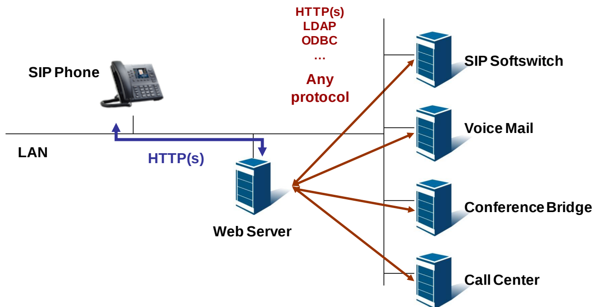
Figure 6: Access to a telephony application
