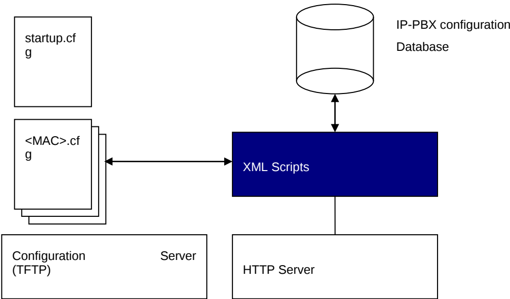
Figure 94: Self-configuration implementation architecture
