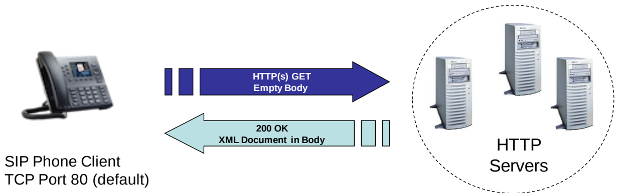
Figure 2: Mitel IP Phone acting as a client
