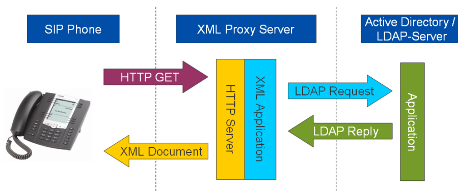
Figure 95: LDAP directory message flow
