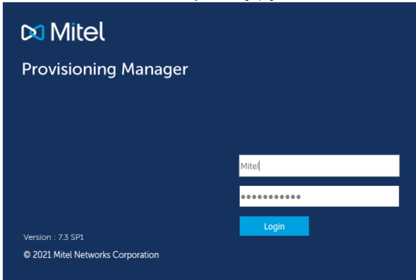
Figure 4.10: Login page
