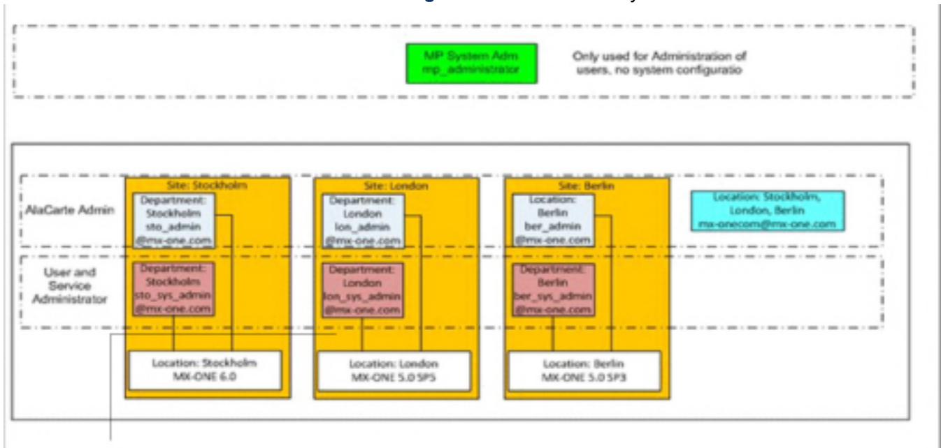
Figure 4.9: User hierarchy
