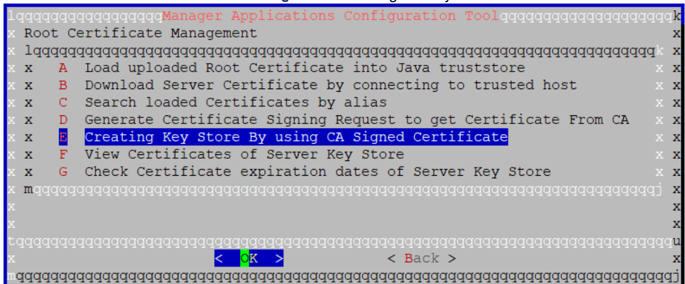
Figure 6.6: Creating the Key Store
