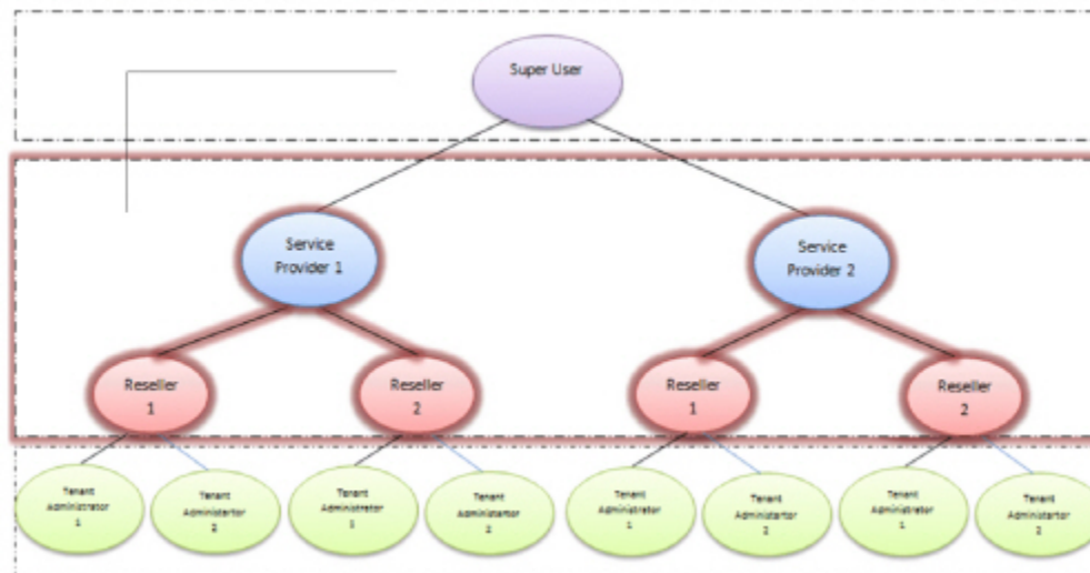
Figure 4.6: Create Reseller
