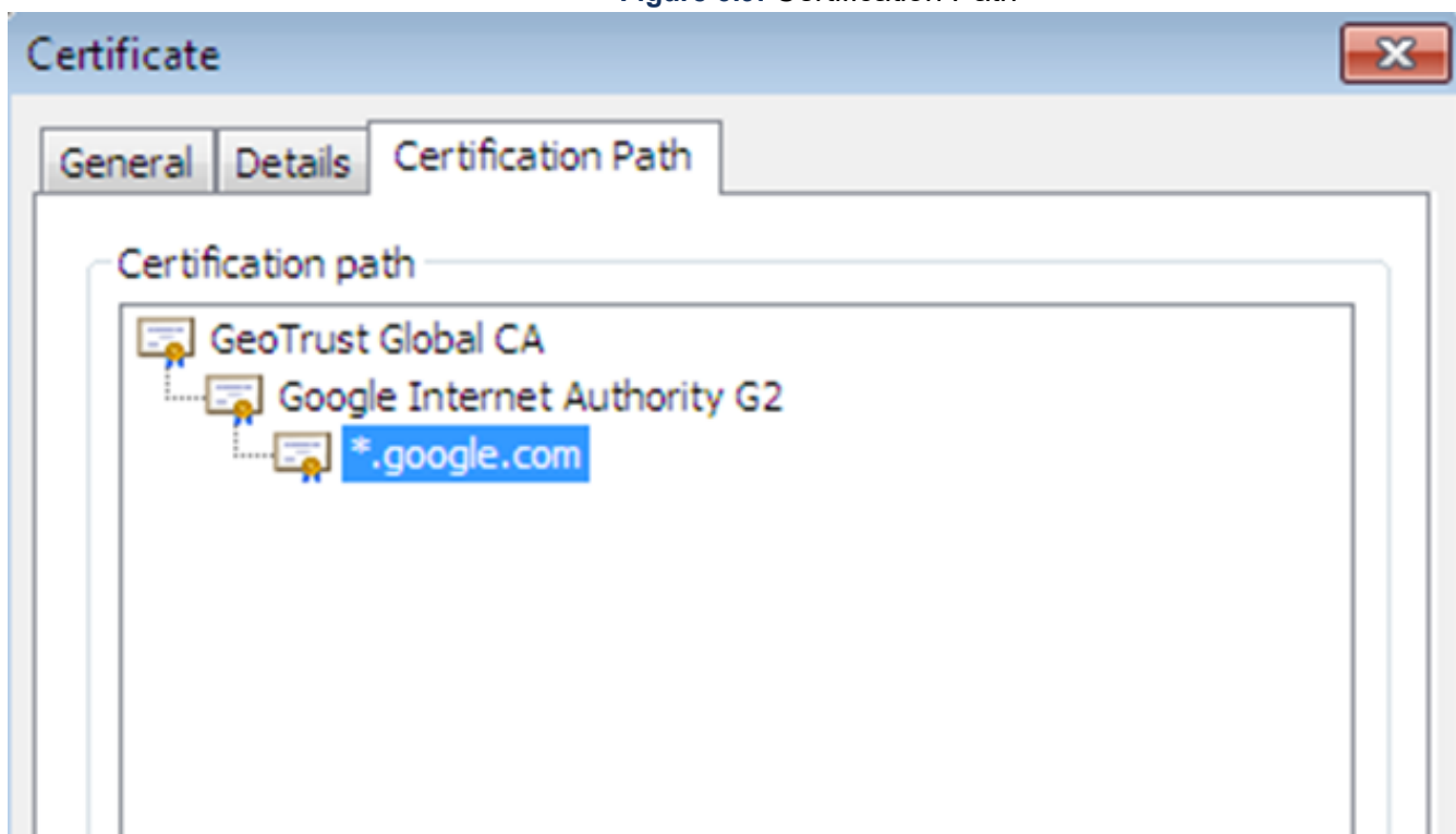
Figure 6.9: Certification Path
