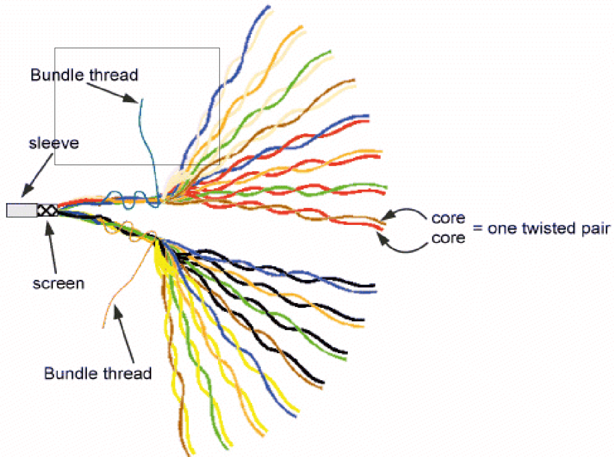
Figure 3.64: Cable Structure
