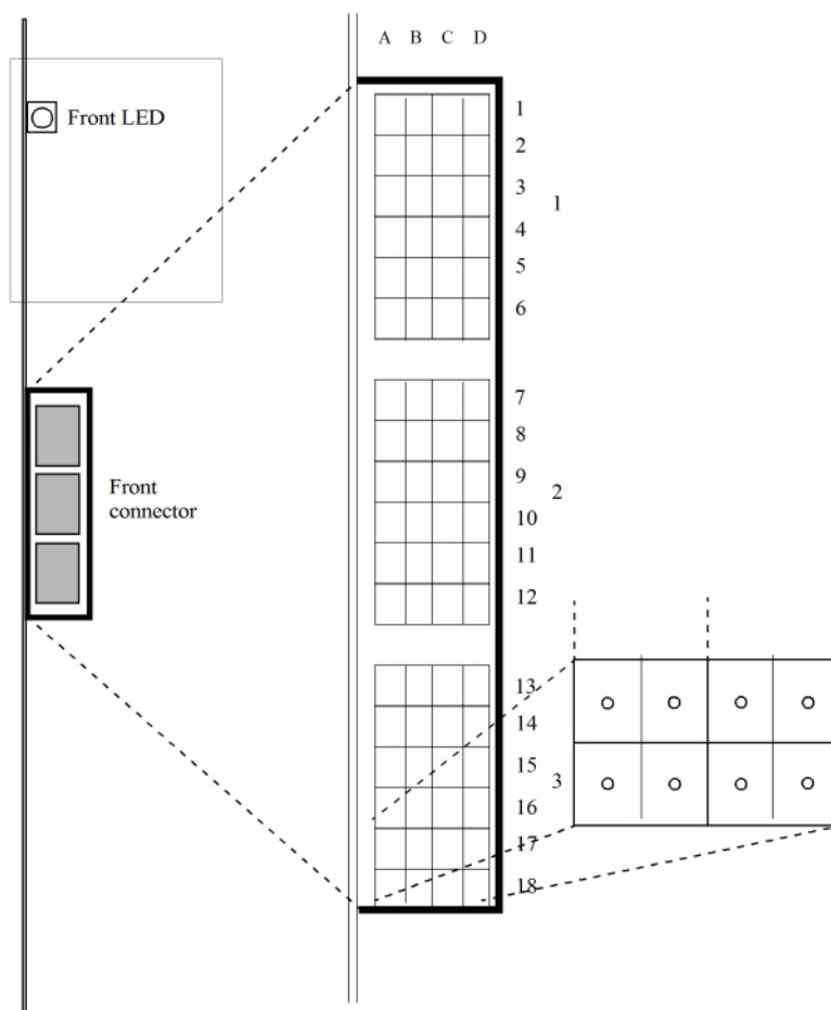
Figure 3.66: Front view
