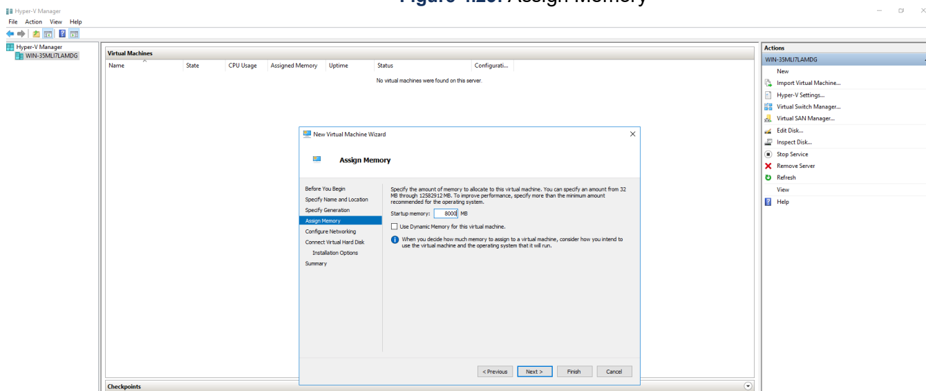
Figure 4.23: Assign Memory
