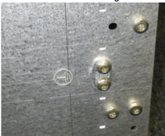
Figure 3.32: Earthing point 7U-chassis
