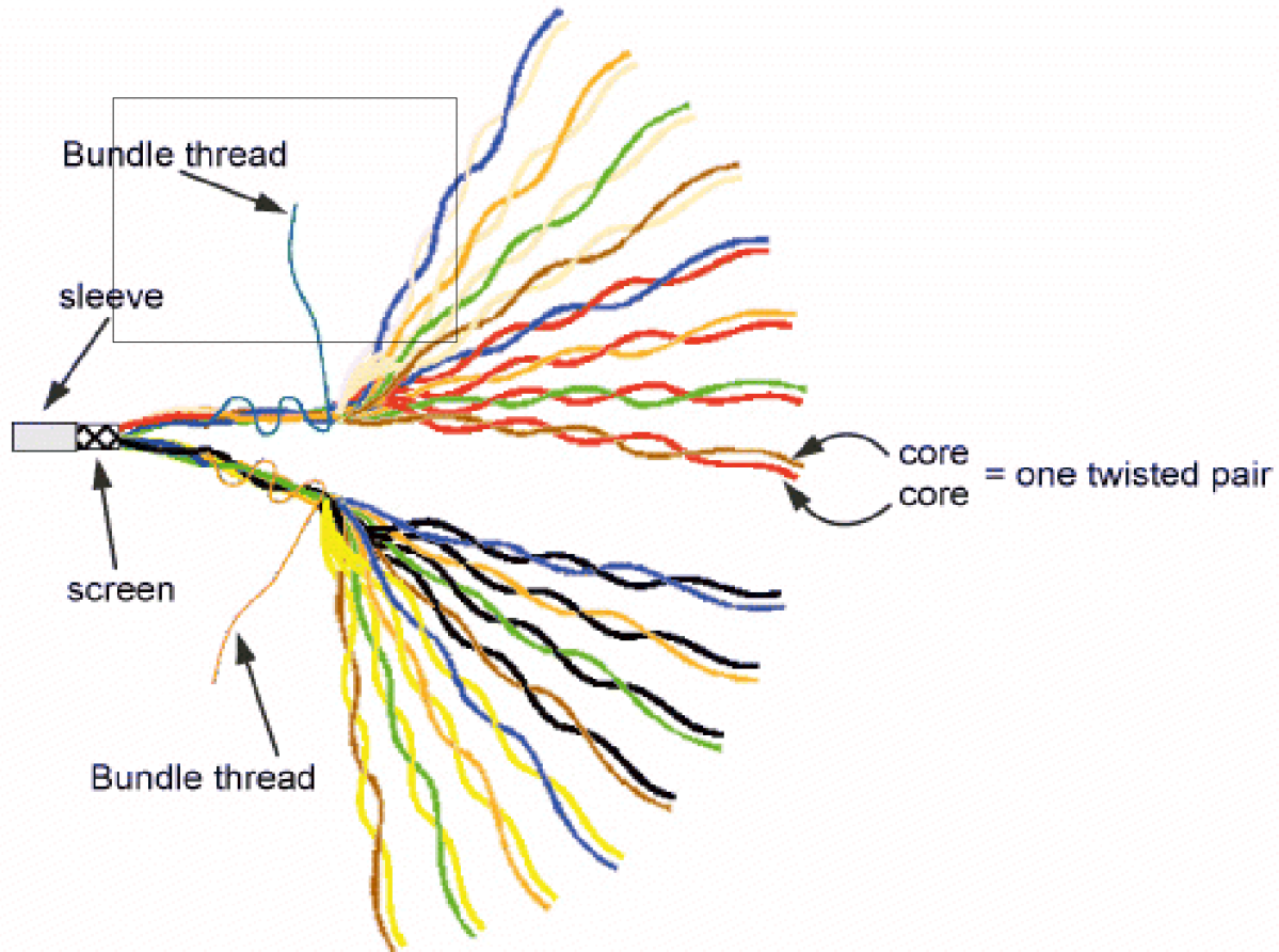
Figure 3.64: Cable Structure
