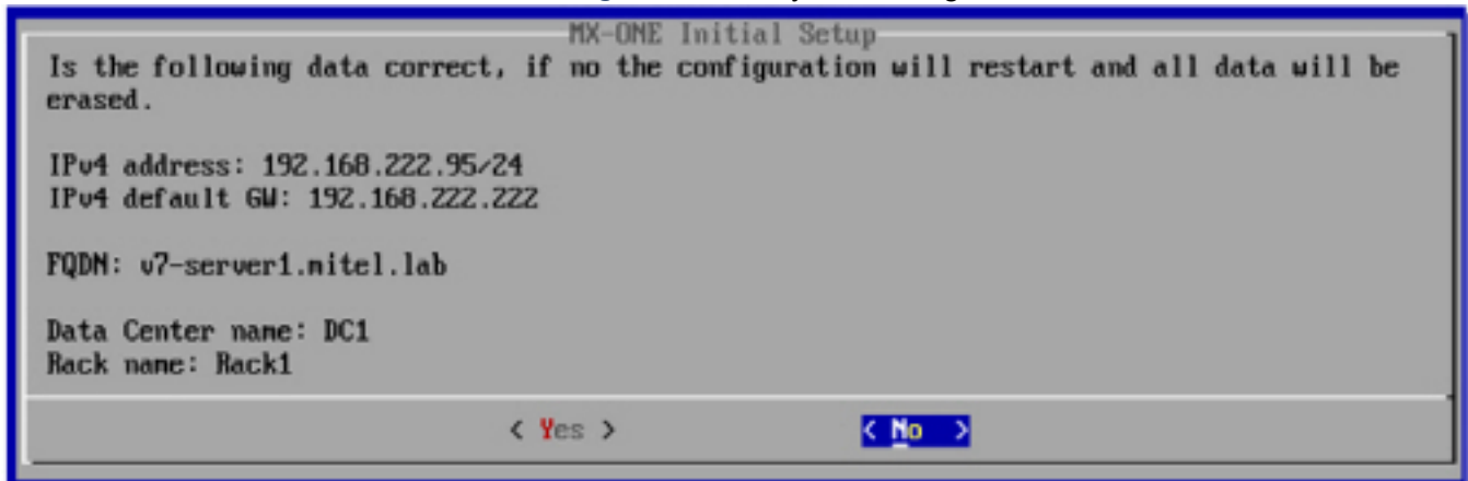
Figure 1.7: Verify the Configuration
