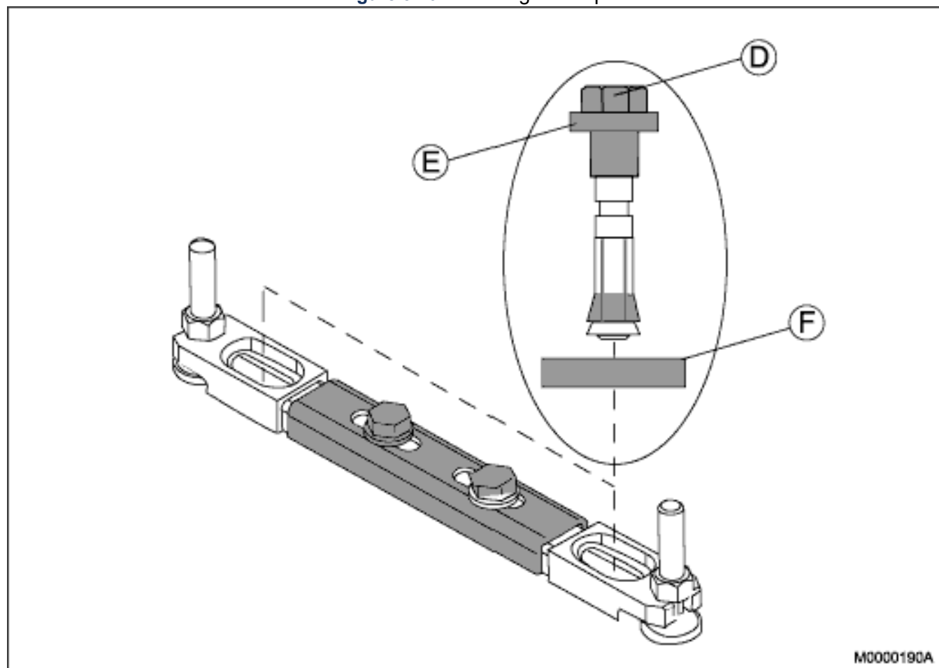
Figure 3.20: Installing the Expander Screw
