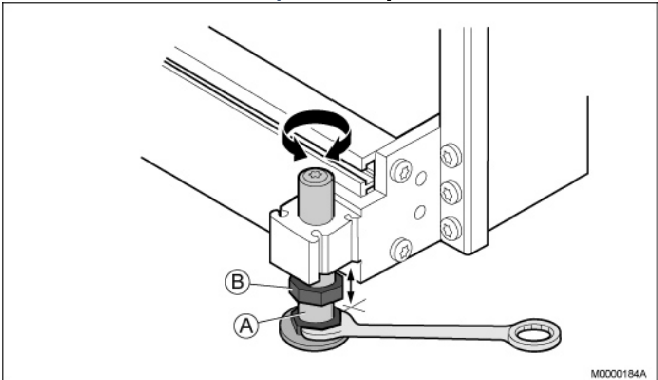
Figure 3.15: Leveling the Cabinet
