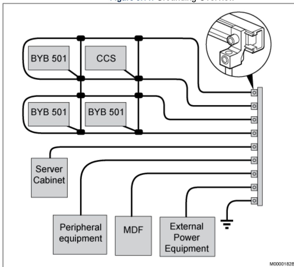
Figure 3.11: Grounding Overview
