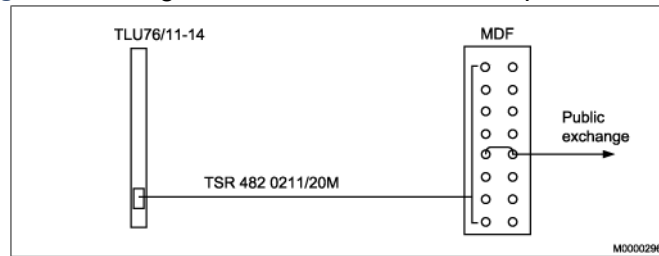
Figure 3.74: Digital external lines 120 ohm pair cable, TLU76/11 - /14
