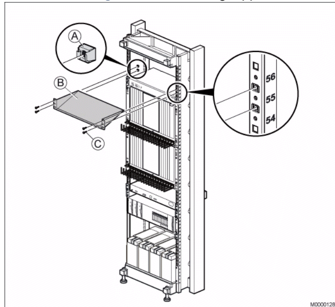
Figure 3.38: Installing Upper Air Plate
