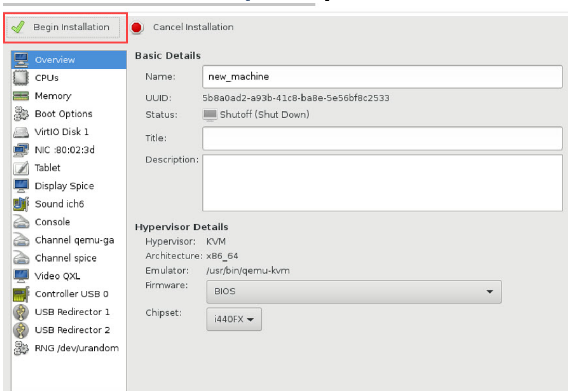
Figure 2.4: Begin Installation
