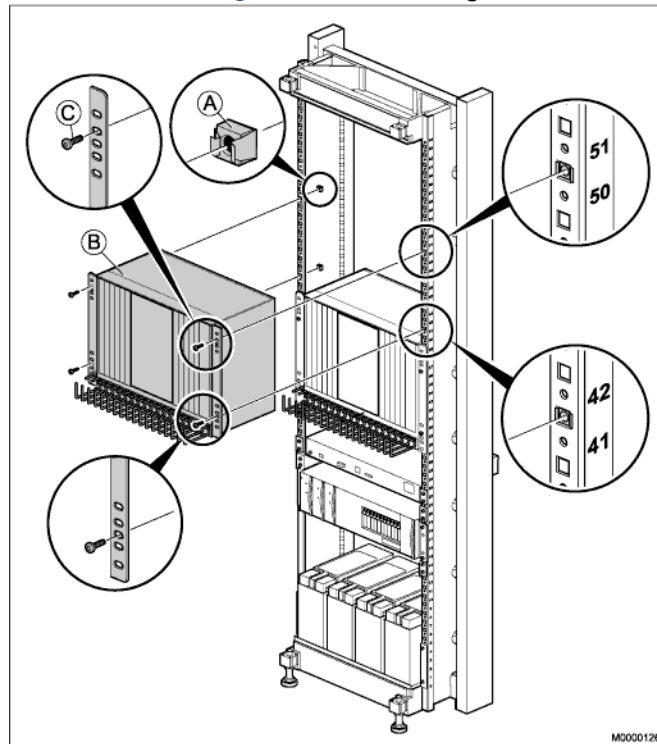
Figure 3.37: Installing Subrack A
