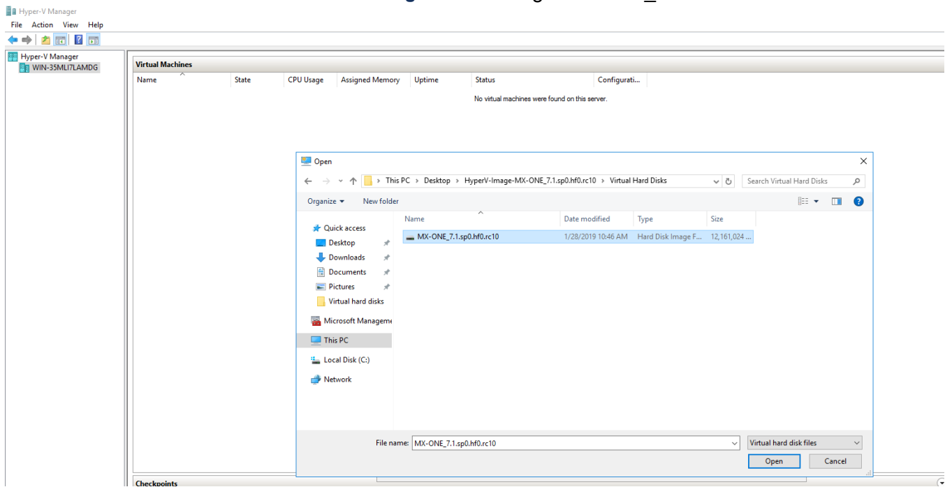
Figure 4.26: Image Selection_2
