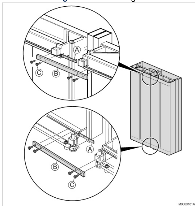
Figure 3.13: Mounting the Earth Bar
