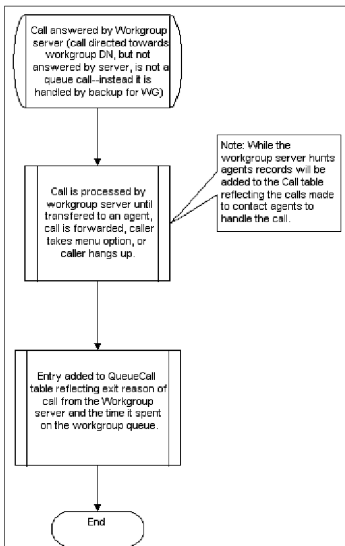
Figure 27 : New Entries to the CallQueue Table
