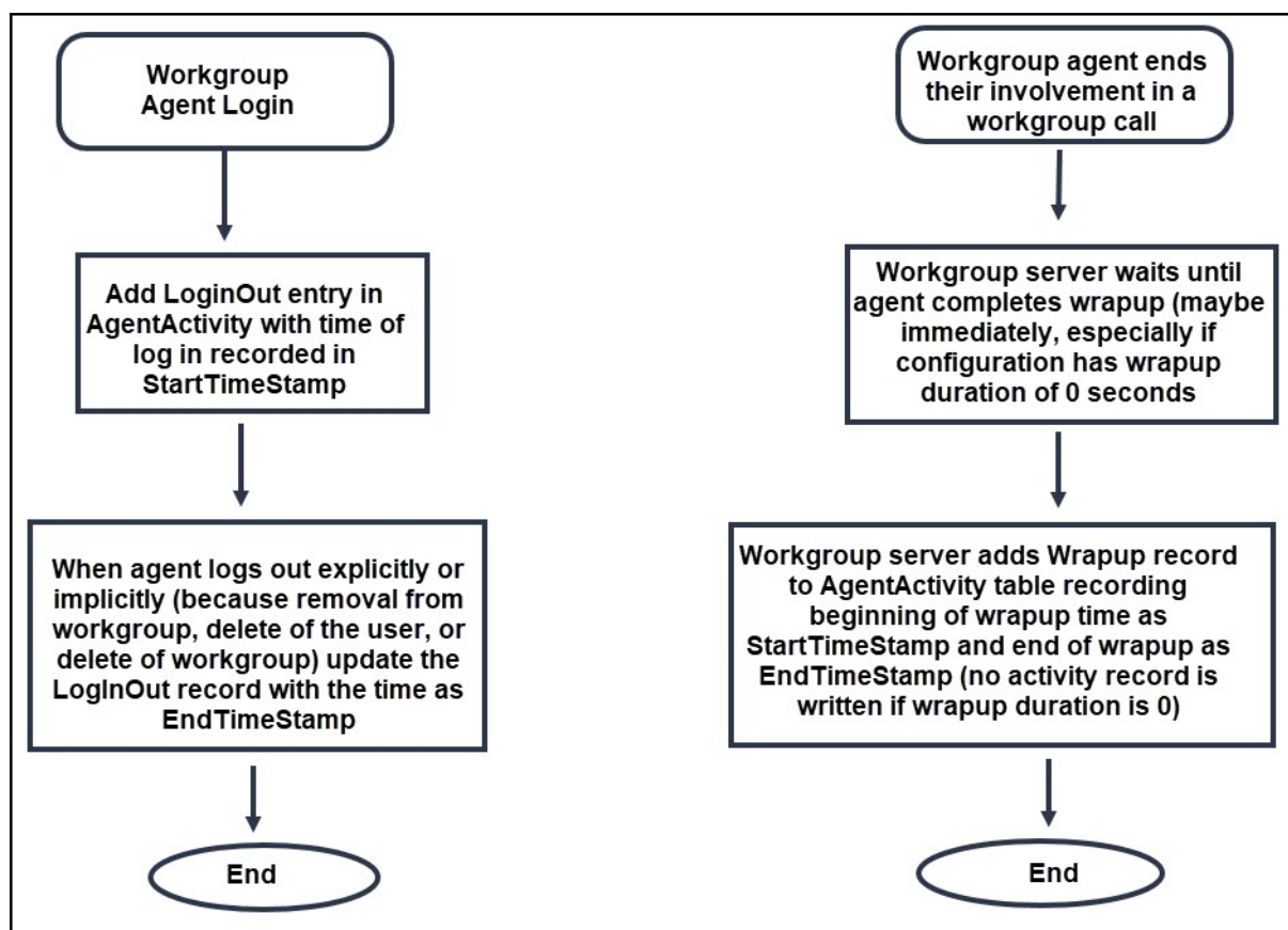
Figure 26 : Entries to the Agent Activity Table
