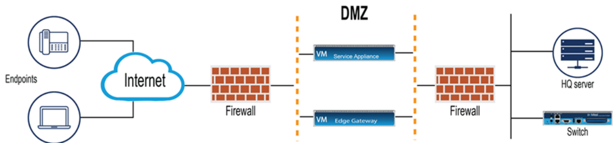
Figure 3 : Service Appliance Deployment for EG
