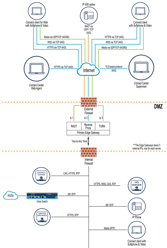
Figure 2 : Network Architecture
