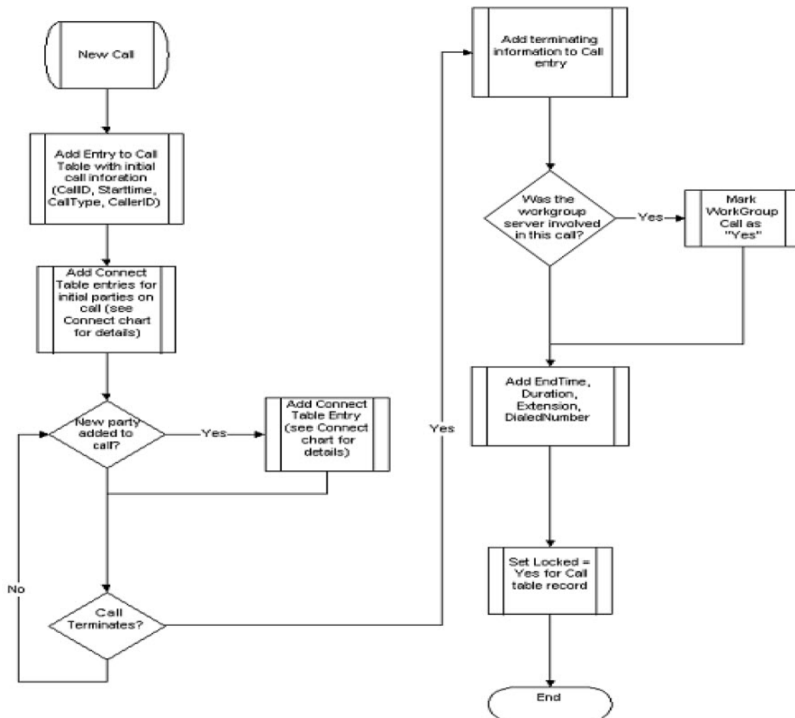
Figure 27 : New Entries in the Call Table
