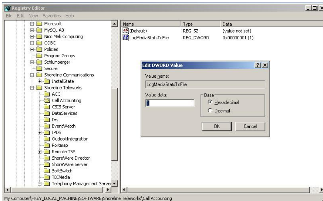
Figure 26 : Value Data Field
