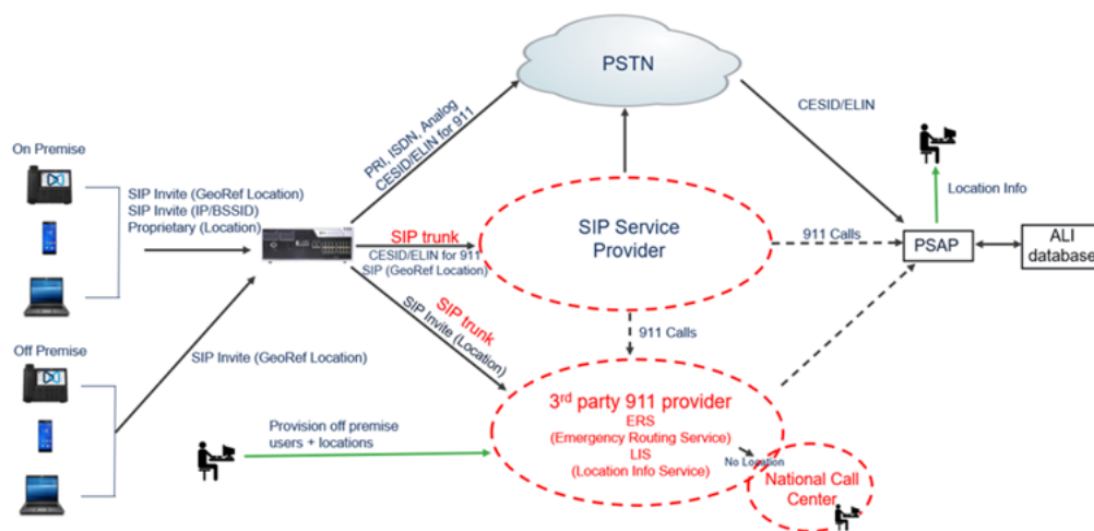
Figure 23 : MiVoice Connect Deployment
