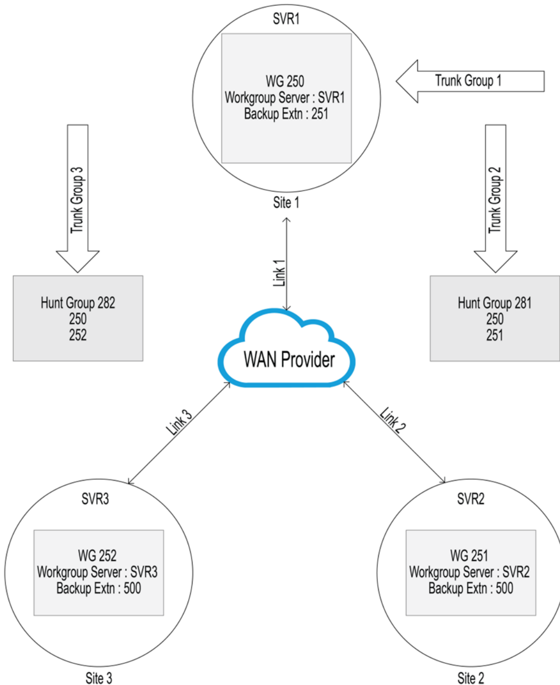
Figure 18 : Hunt Groups Supporting Distributed Workgroups
