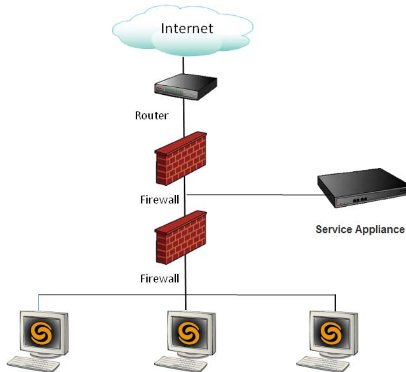
Figure 4.2: Deploying a service appliance in DMZ
