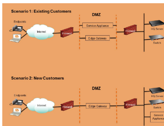
Figure 3 : Service Appliance Deployment for EG
