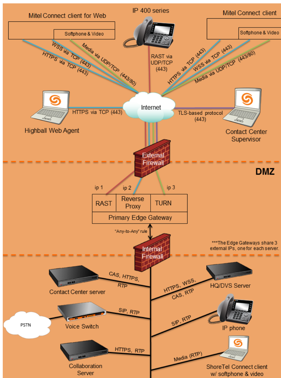
Figure 2 : Network Architecture
