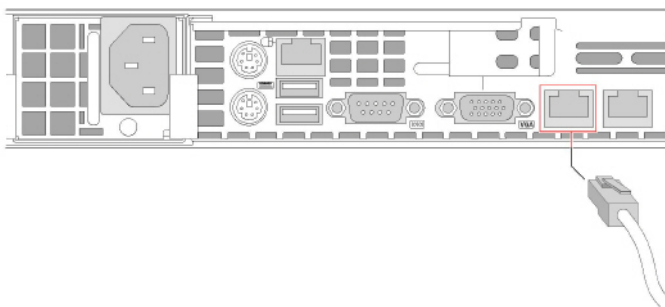
Figure 9 : Connecting the Ethernet Cable to the SA400
