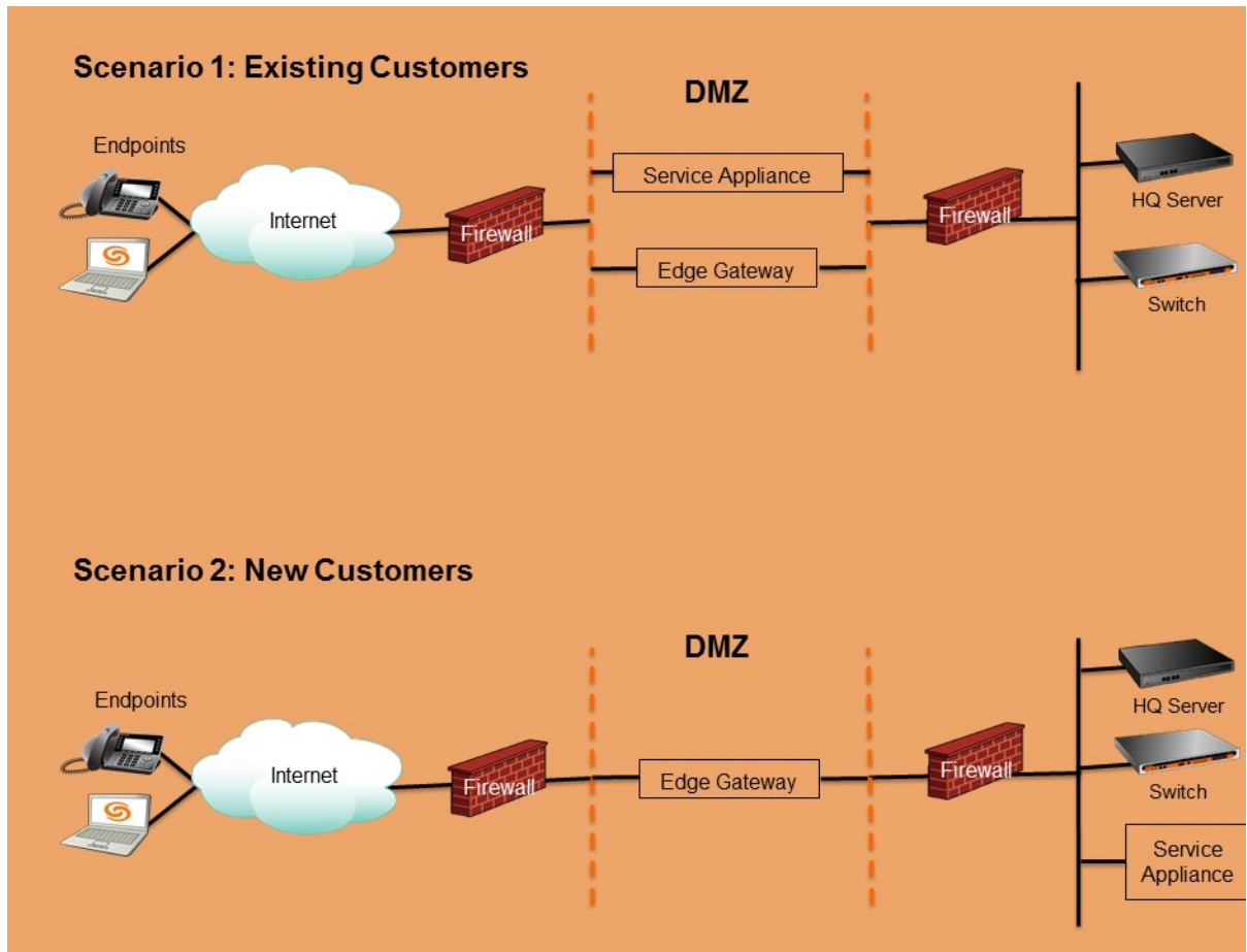
Figure 3.3: Service Appliance Deployment for EG
