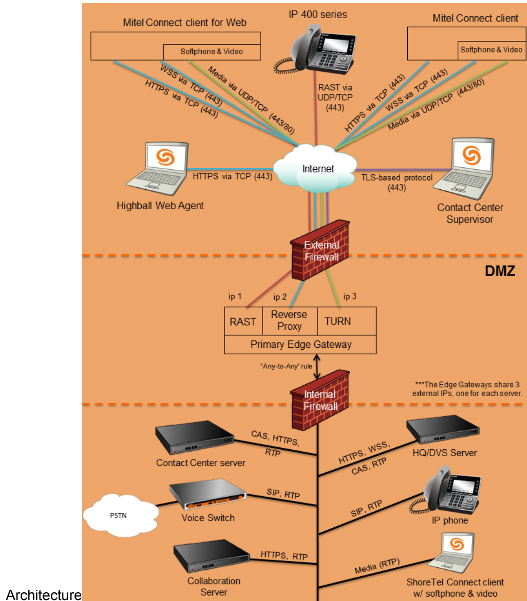
Figure 3.2: Network
