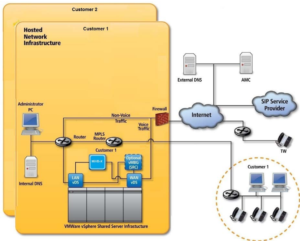
Figure 1: Hosting Remote Office via MPLS (Network Edge)
