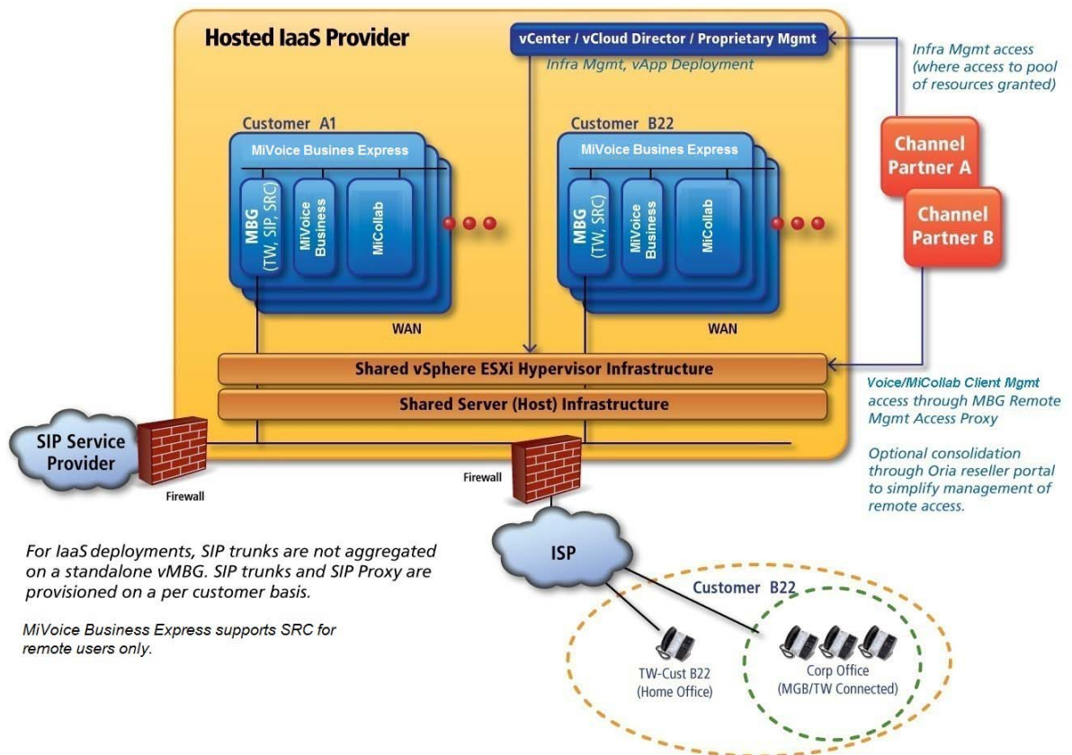
Figure 6: IaaS Infrastructure: Public Internet Connected End Customer(s)
