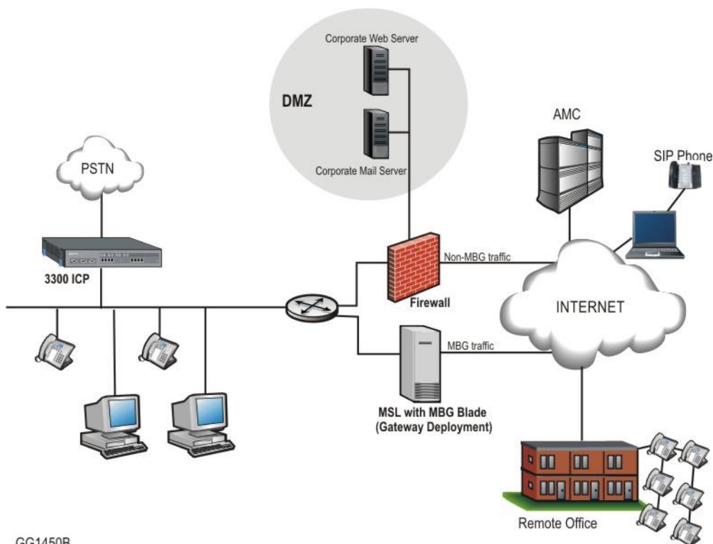
Figure 1. Server-Gateway Configuration
