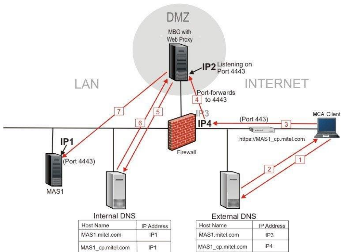
Figure 14. Message Flow for Web Conferencing Requests
