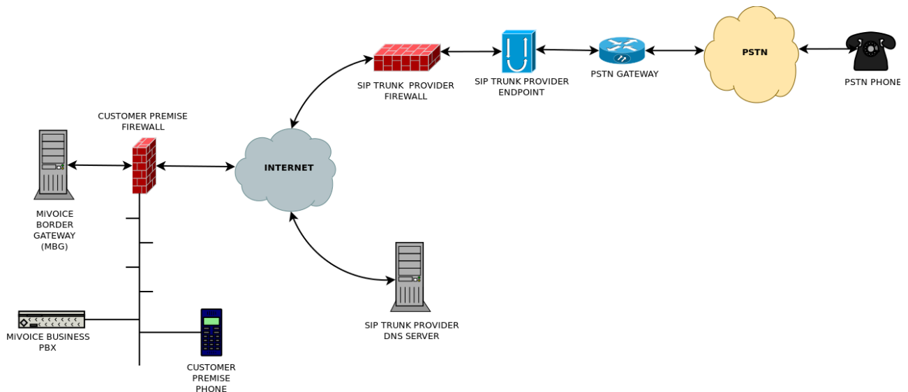
Figure 9: SIP Trunking
