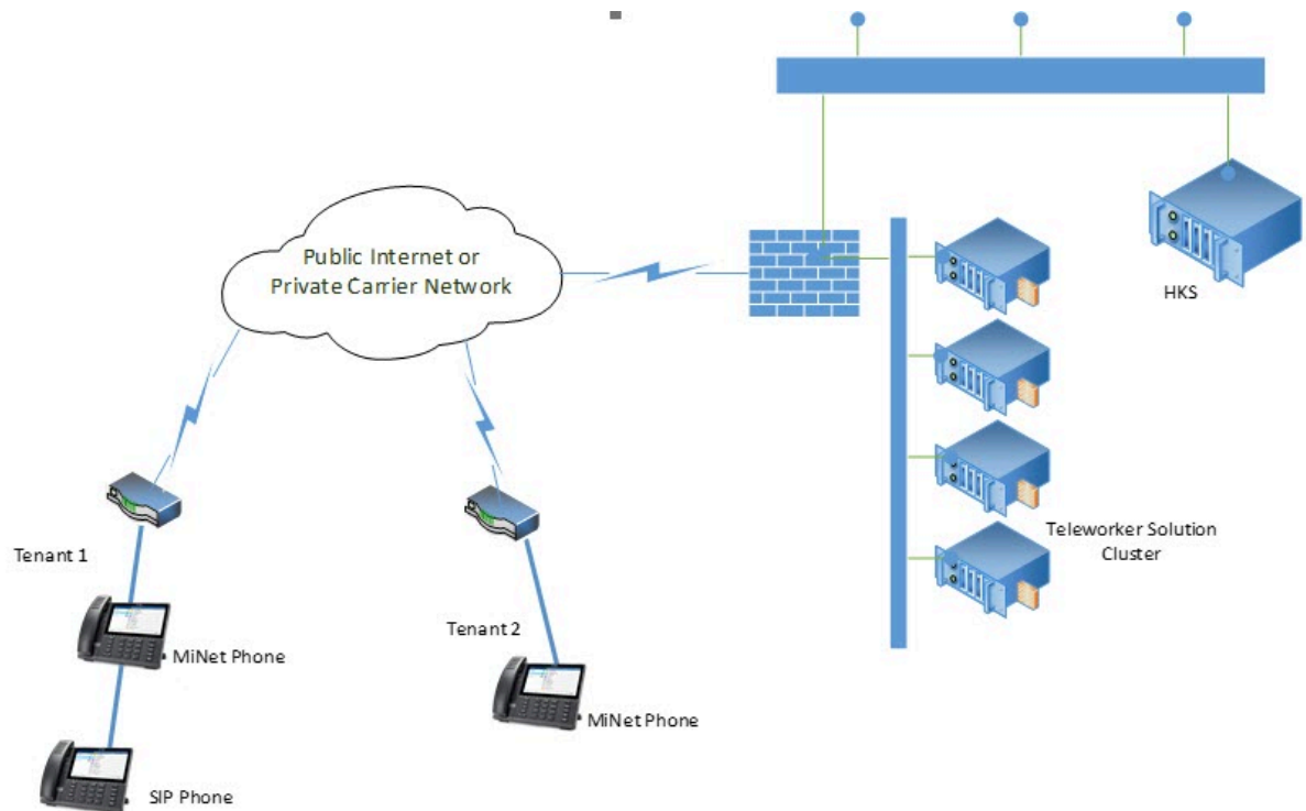
Figure 7: MBG as a Gateway for Broadview Networks Silhouette
