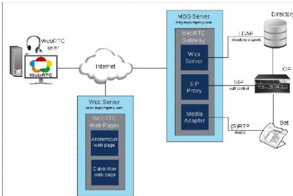
Figure 15: WebRTC Gateway and Web Pages Topology
