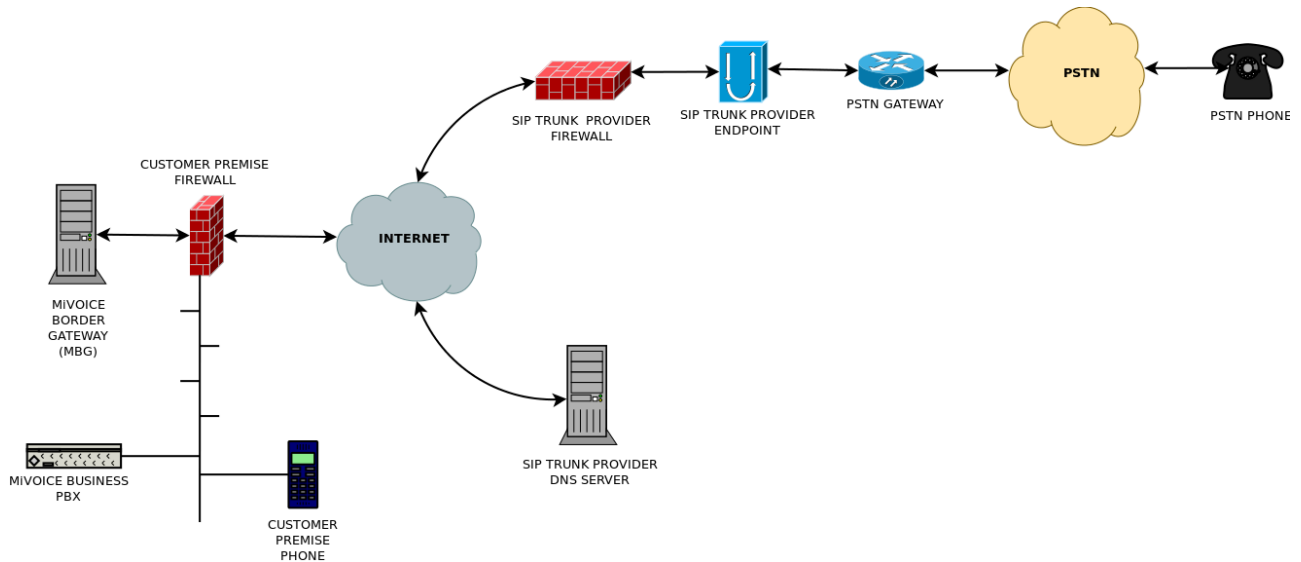
Figure 10: SIP Trunking
