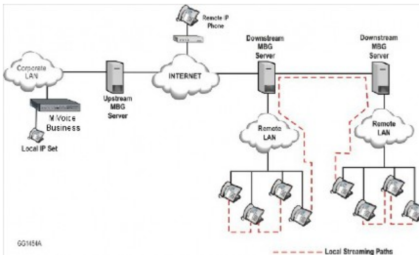
Figure 13: Multiple downstream MBGs
