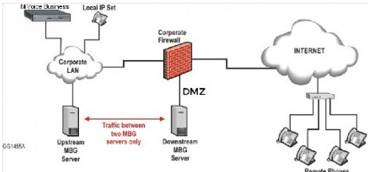
Figure 11: Daisy-chained MBGs for enhanced security
