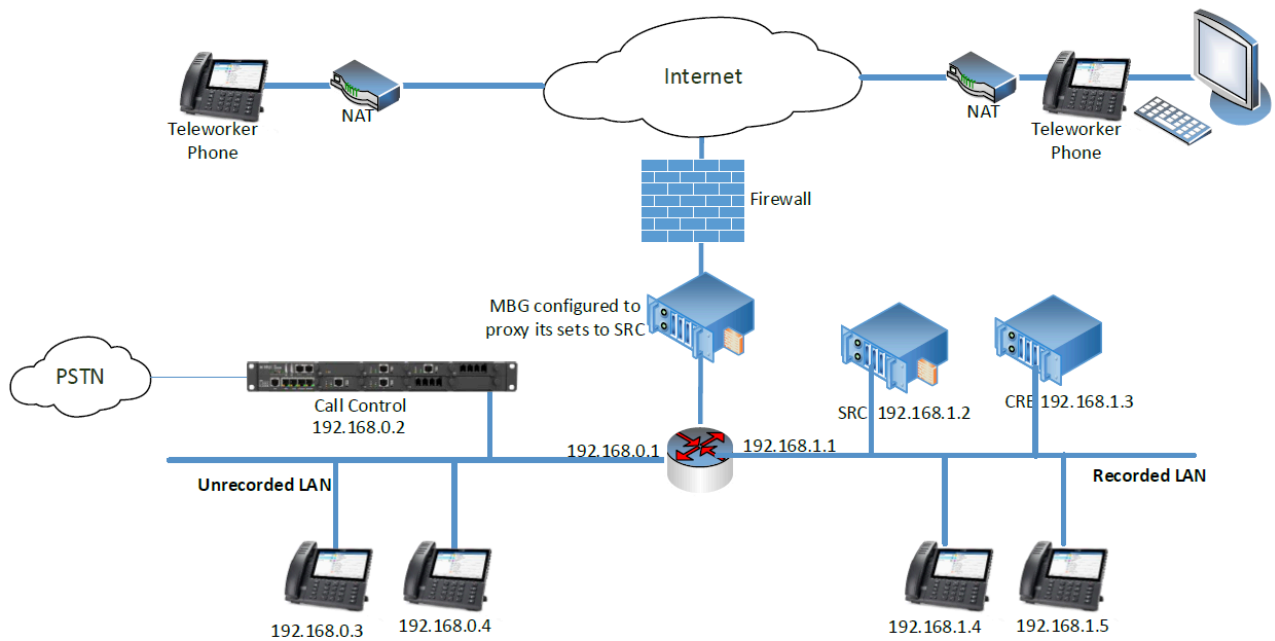
Figure 9: Recording Teleworker Sets
