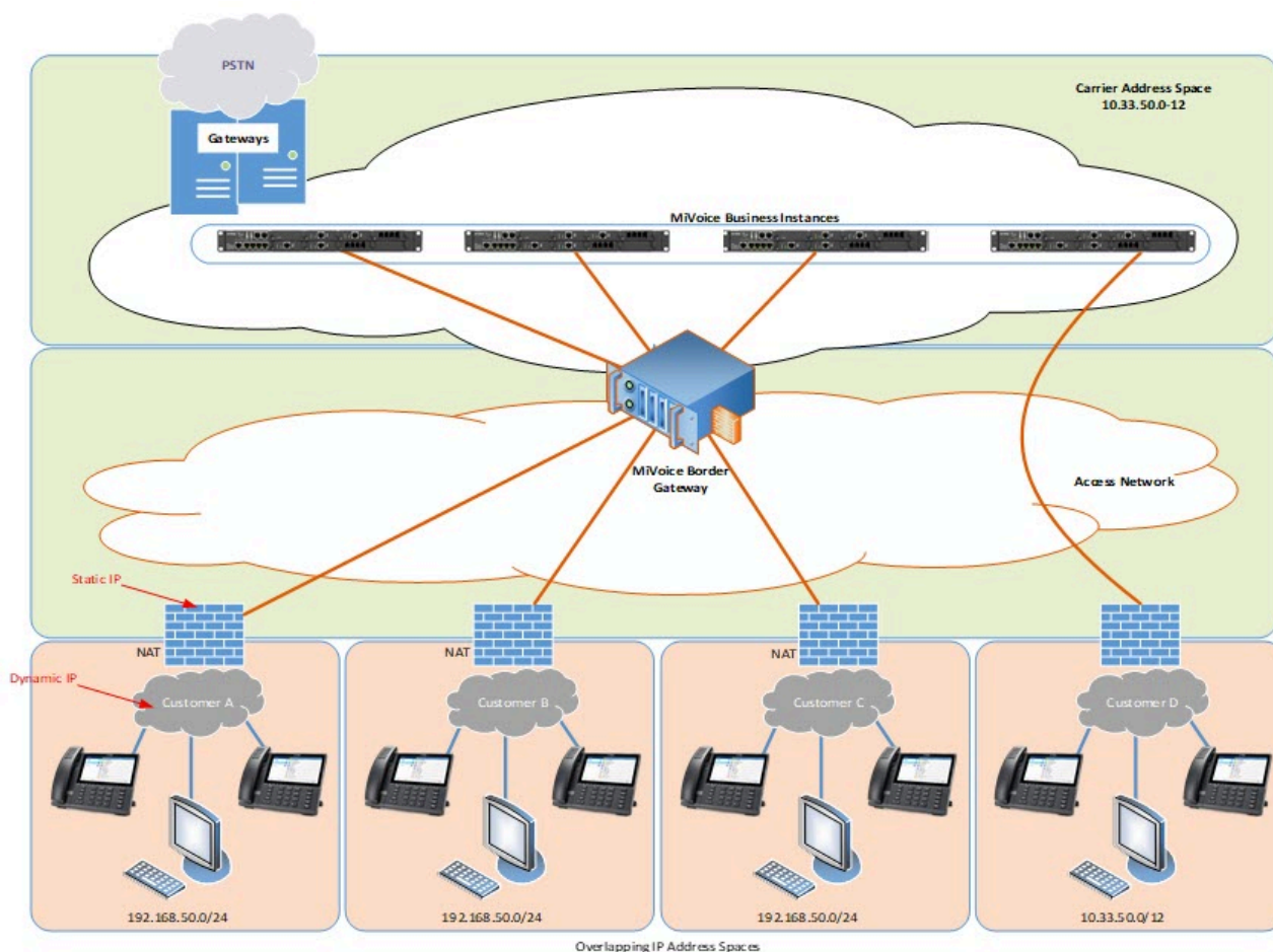
Figure 6: MBG providing NAT traversal to multiple MiVoice Business instances
