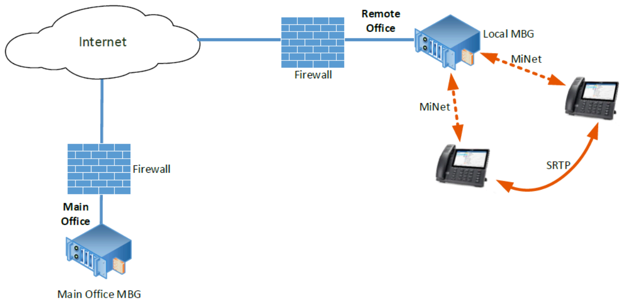
Figure 12: Daisy-chained MBGs to save bandwidth
