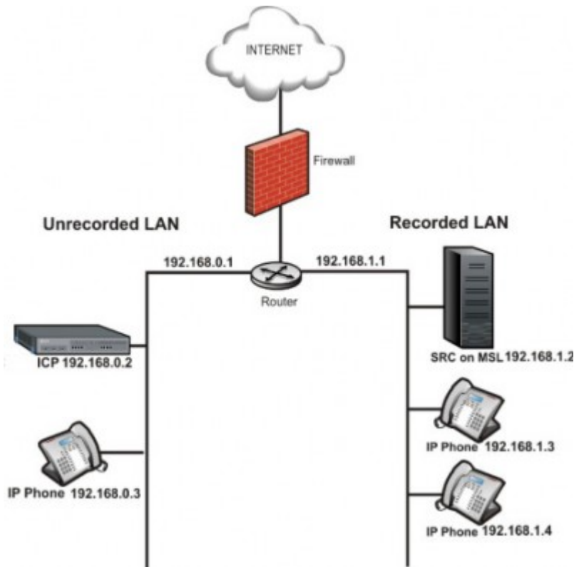
Figure 6: MBG Deployed on the LAN for Call Recording
