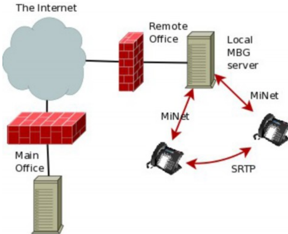
Figure 9: Daisy-chained MBGs to save bandwidth
