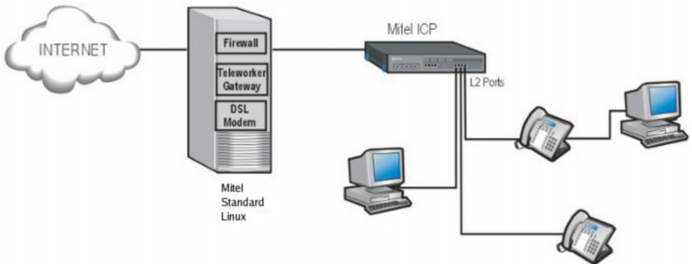
Figure 2: MBG as Internet Gateway (no enterprise firewall)
