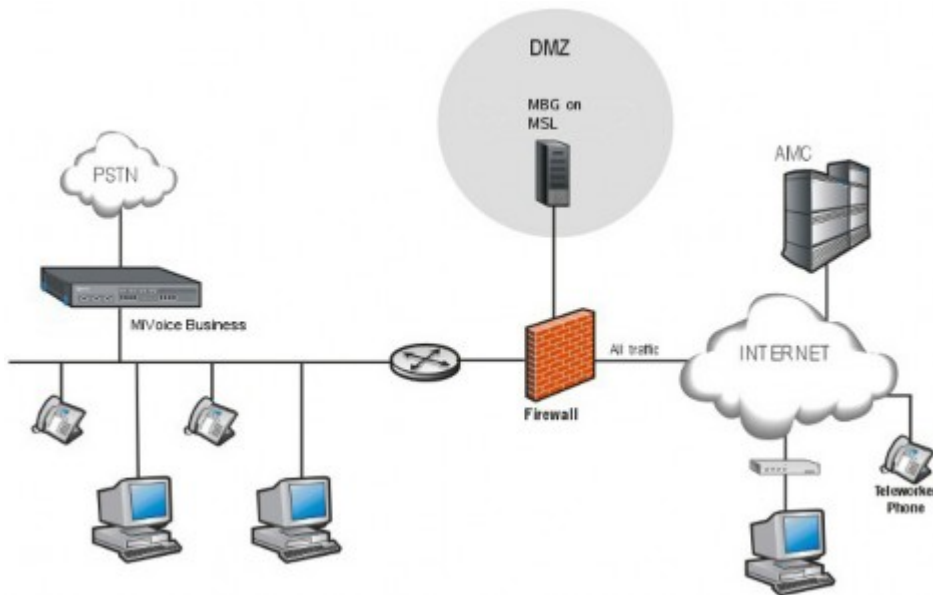
Figure 3: MBG deployed in a DMZ
