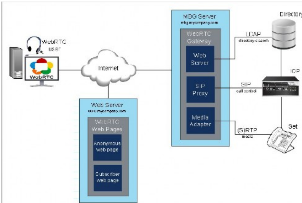
Figure 12: WebRTC Gateway and Web Pages Topology
