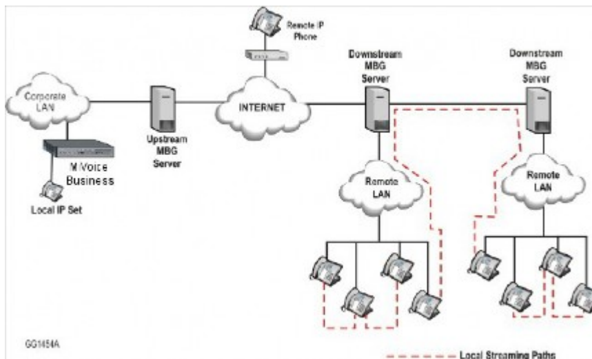
Figure 10: Multiple downstream MBGs
