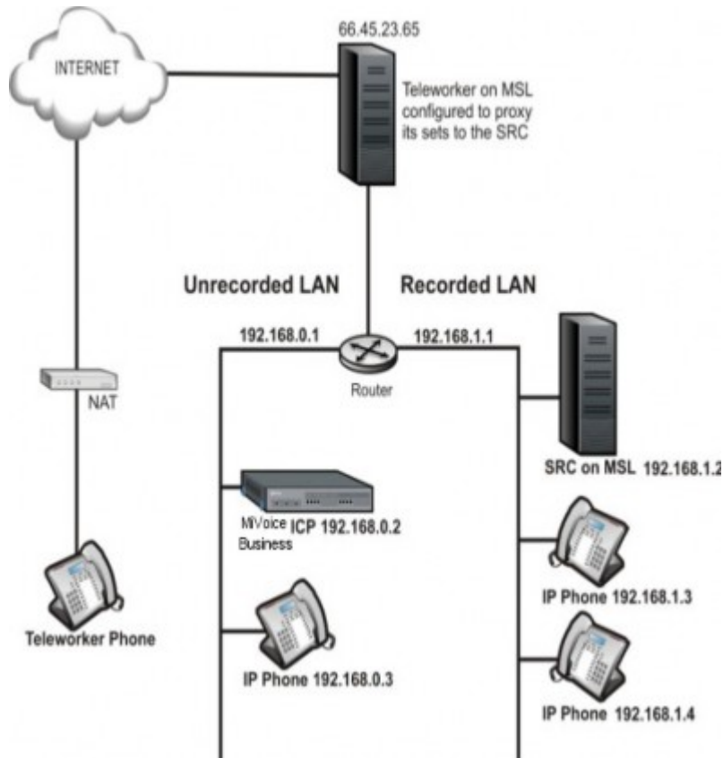
Figure 7: Recording Teleworker Sets
