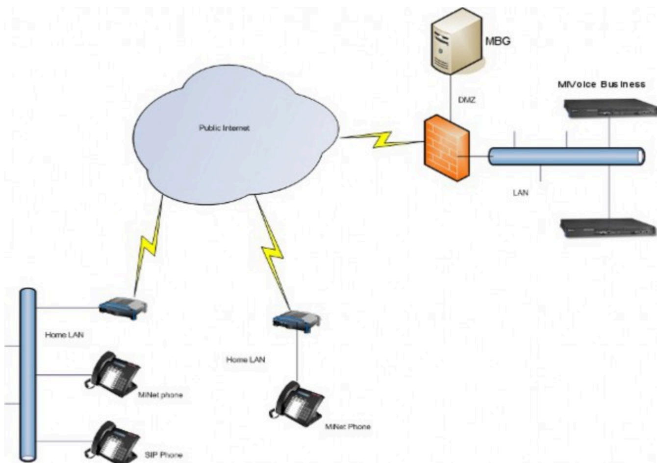
Figure 1: MBG in traditional Teleworker configuration
