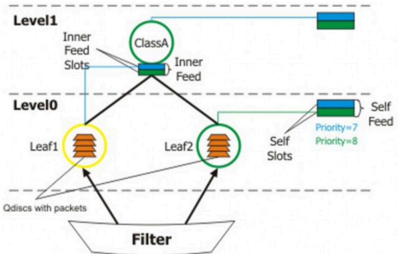
Figure 13: The Hierarchical Token Bucket Queue
