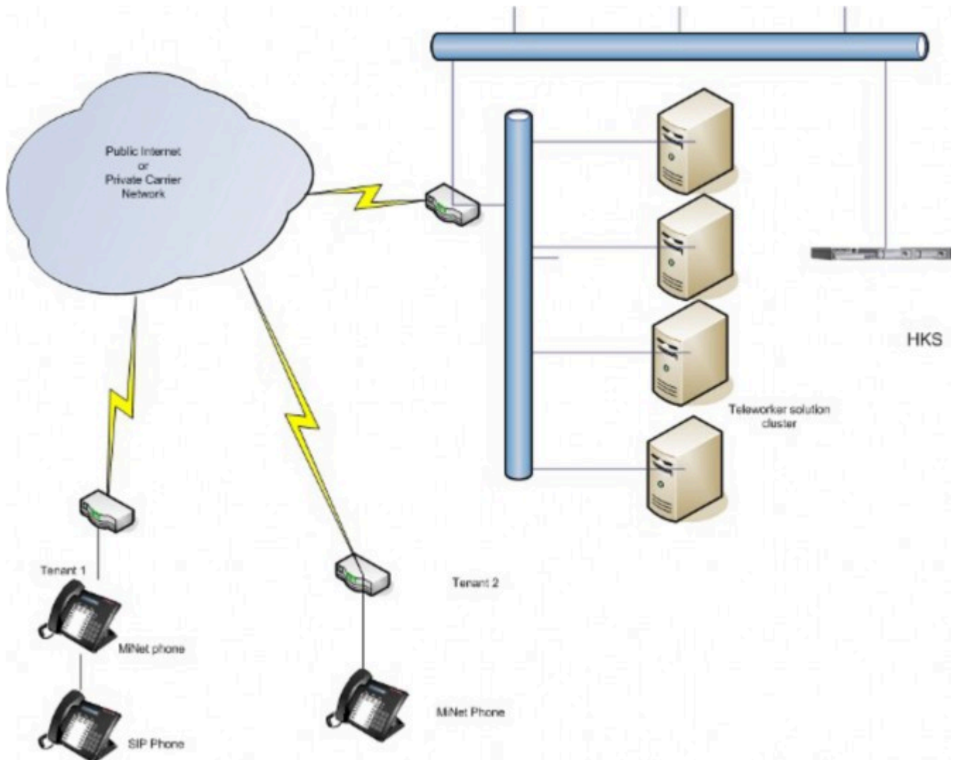
Figure 5: MBG as a Gateway for Broadview Networks silhouette
