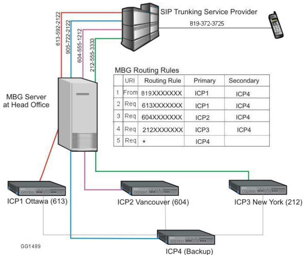
SIP Trunking Configuration Example with DID Routing Rules
