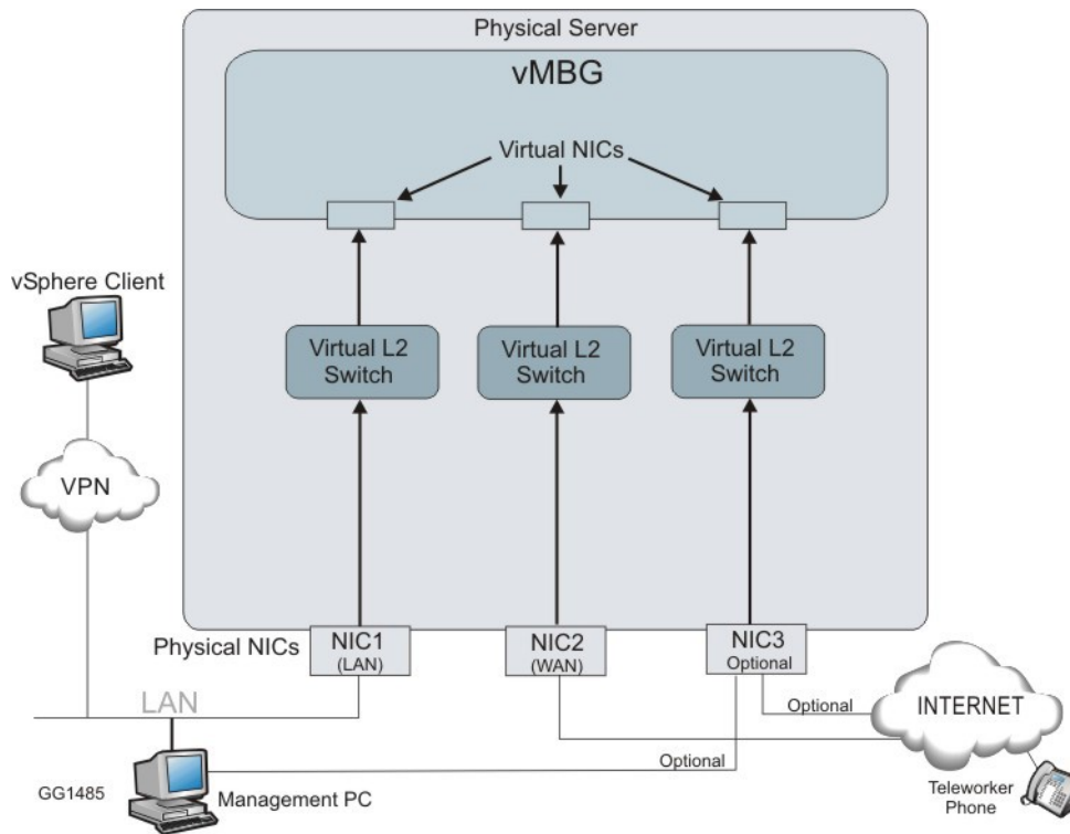
Typical Virtual MBG Appliance
