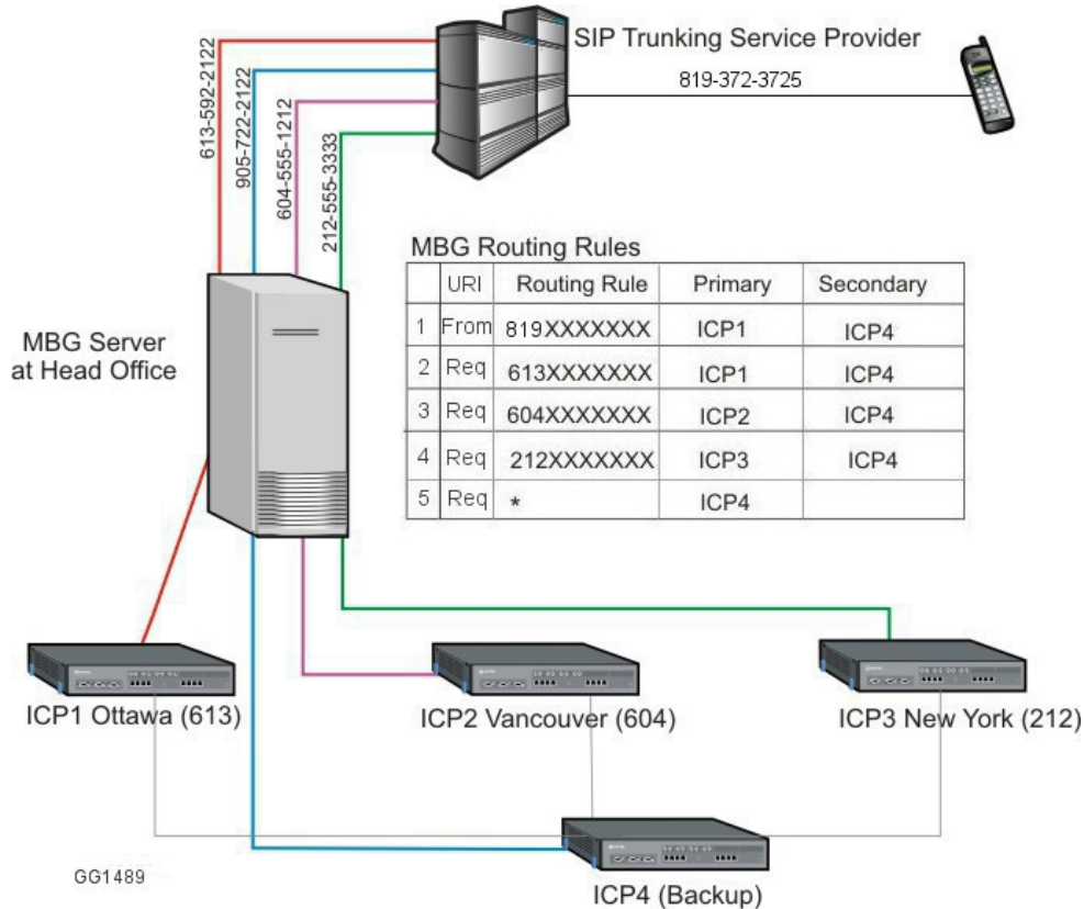
SIP Trunking Configuration Example with DID Routing Rules
