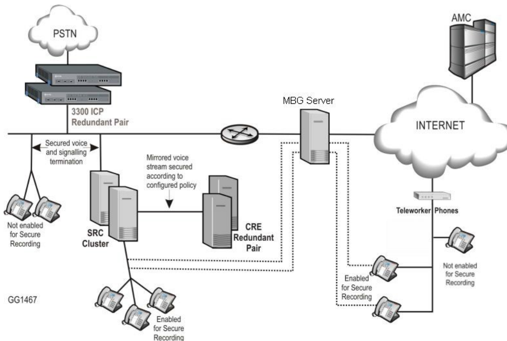
MBG Server with SRC Service (Direct Call Recording)
