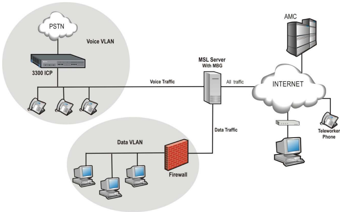
Server-gateway with Bridged Interface Configuration
