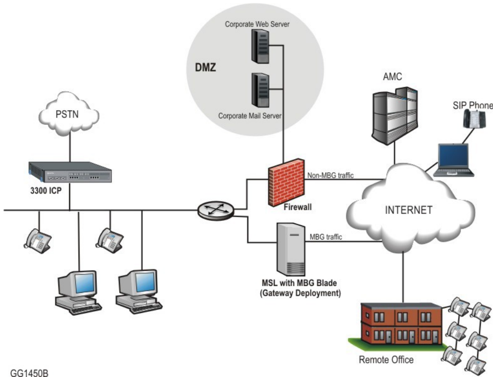
Server-Gateway Configuration
