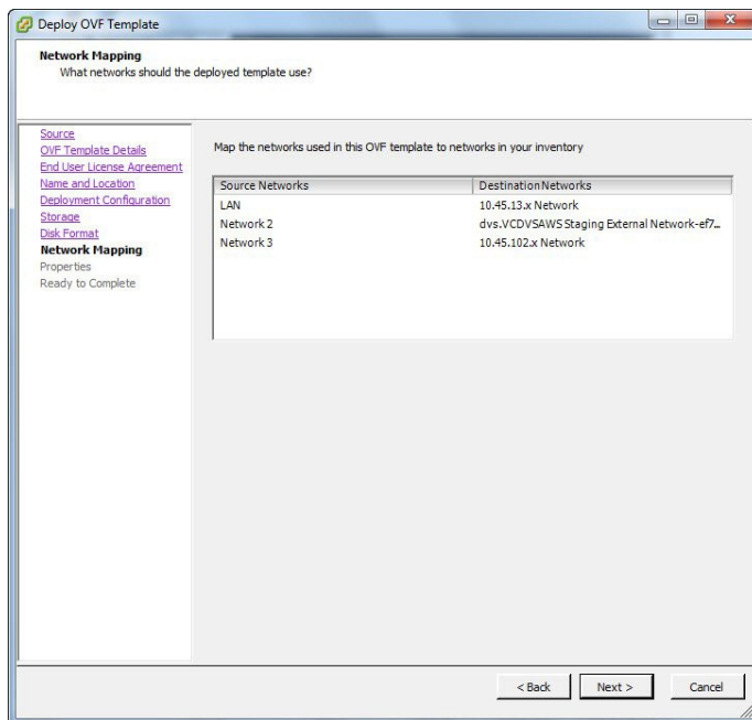
Network Mapping
