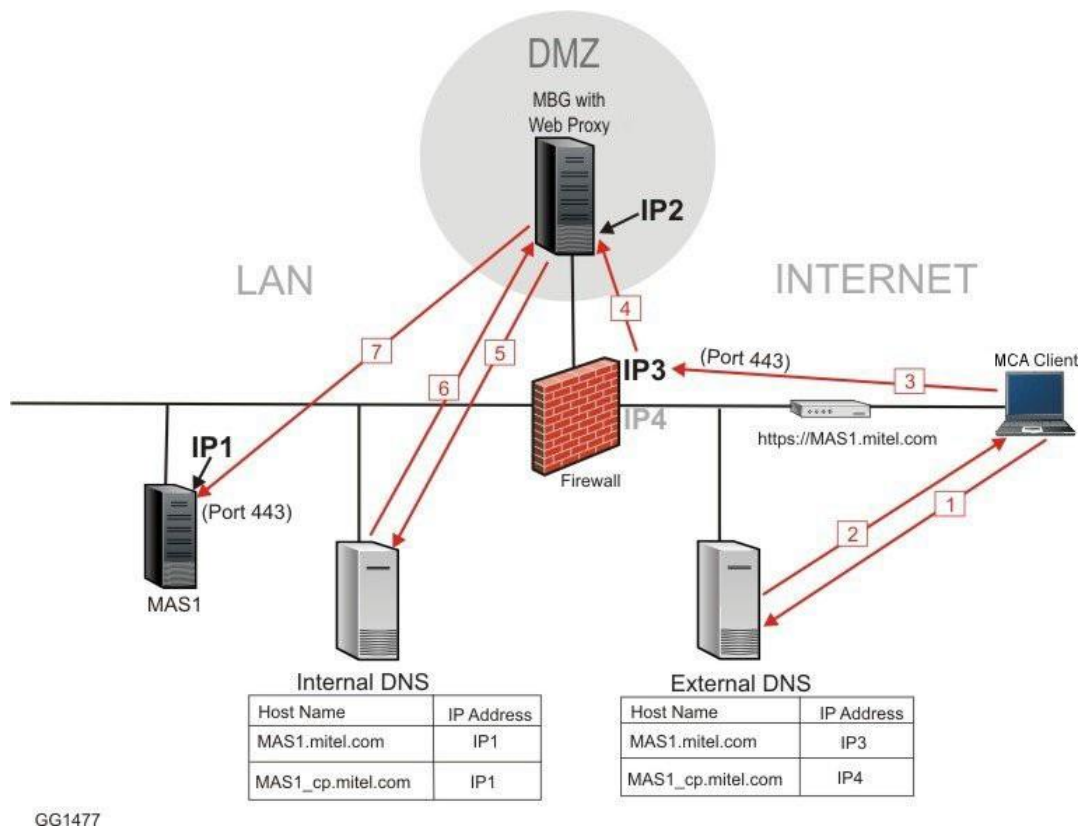
Figure 134. Message Flow for Web Traffic
