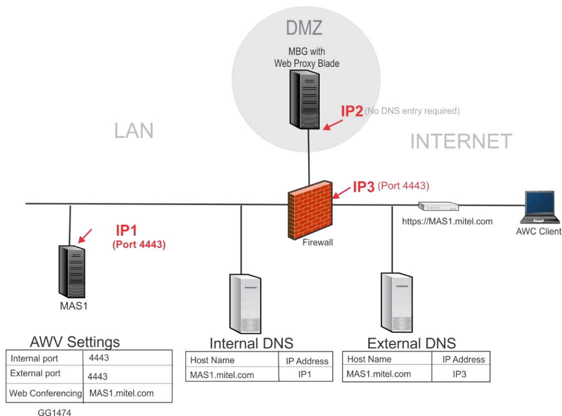
Figure 13: AWW Configuration with Dedicated TCP Port on Primary External IP Address
