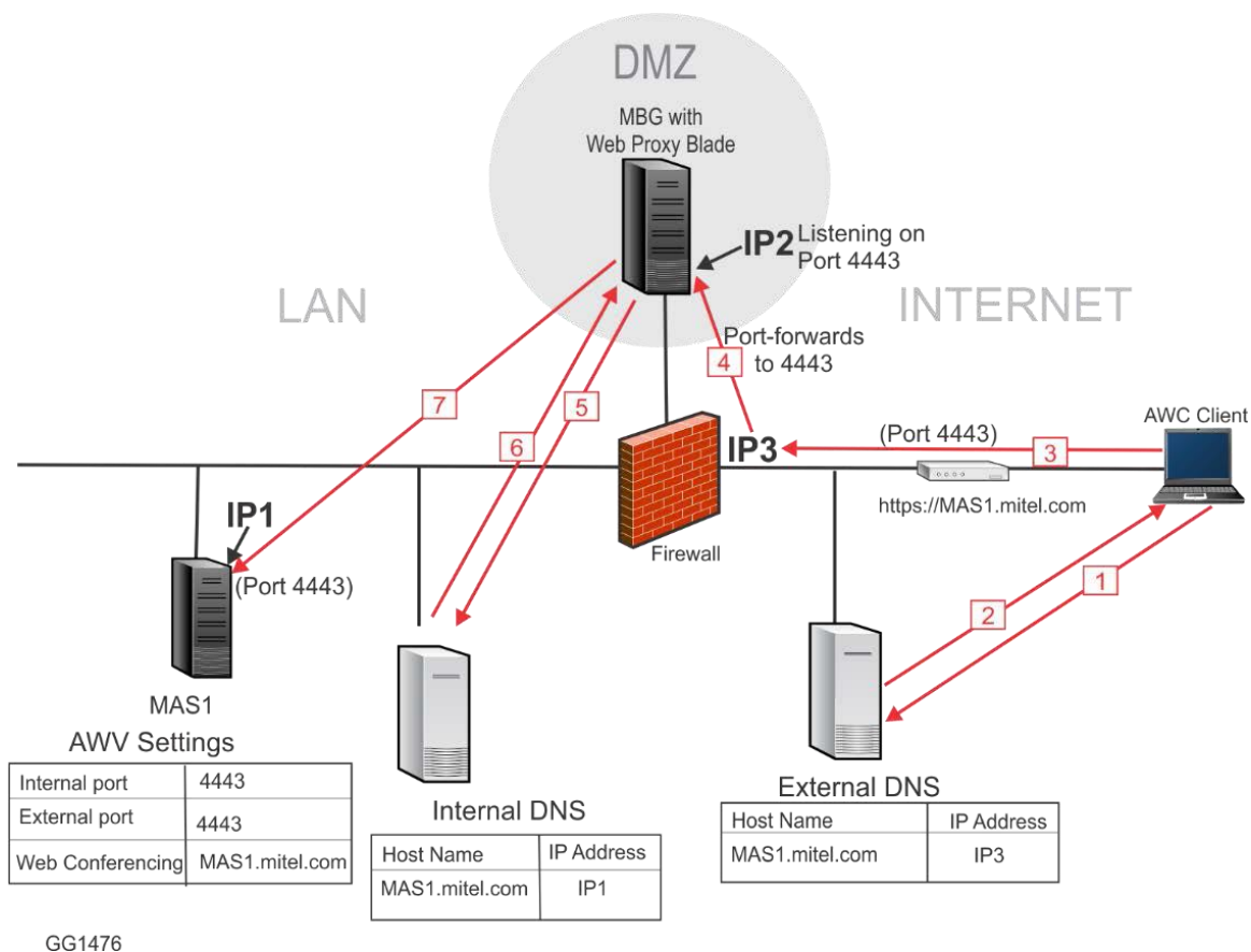
Figure 16. Message Flow for Web Conferencing Requests with One IP
