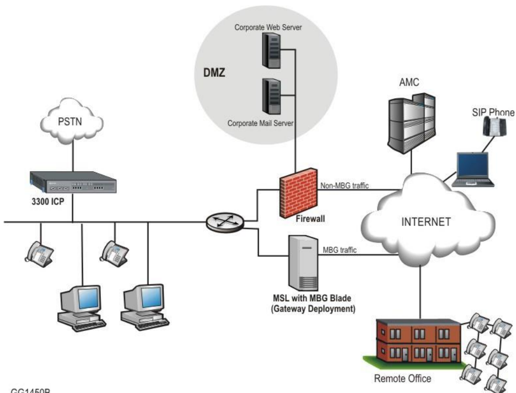
Figure 1. Server-Gateway Configuration
