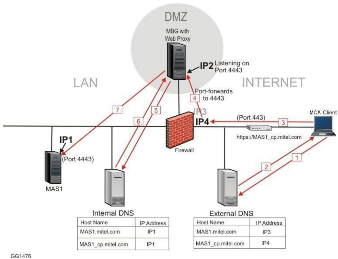
Figure 145. Message Flow for Web Conferencing Requests with Two IPs
