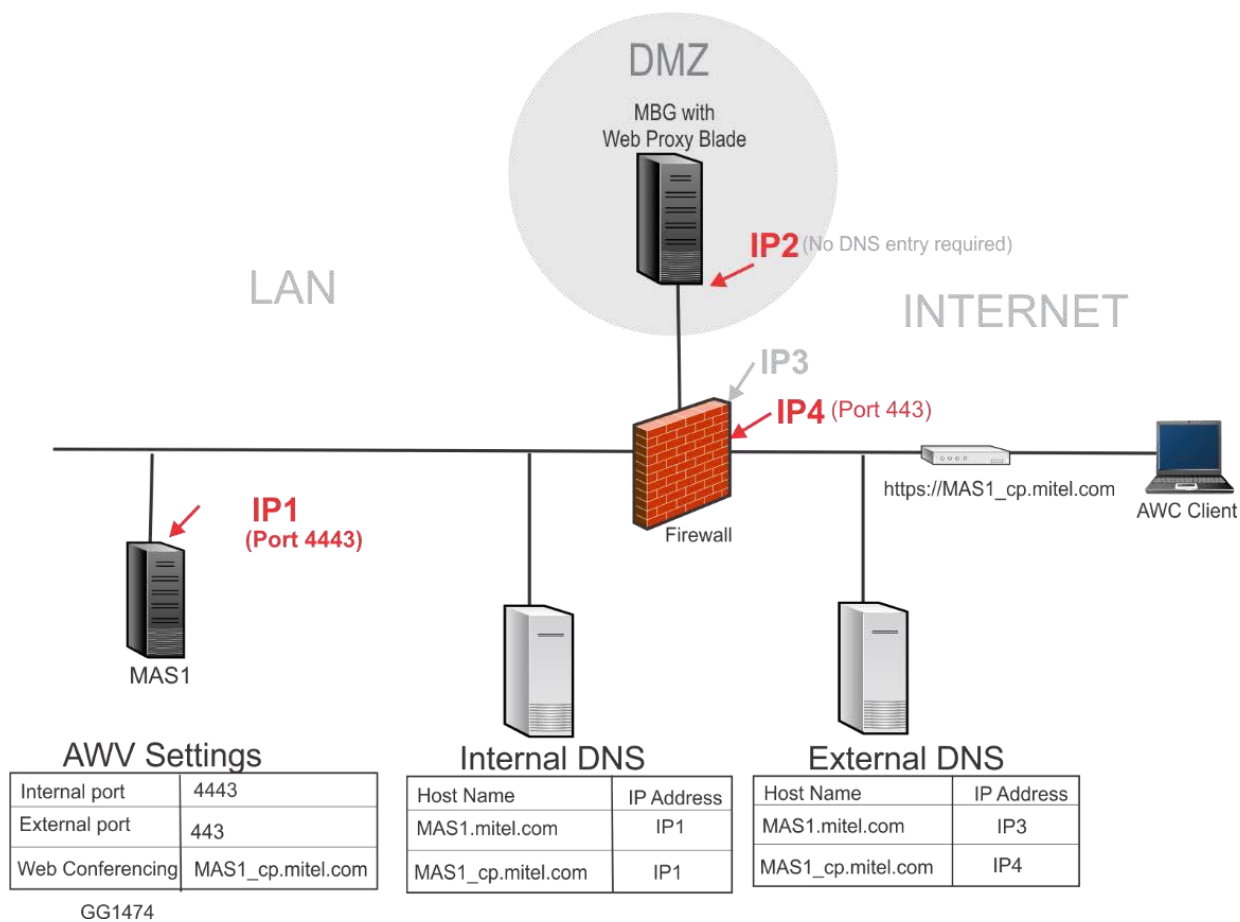
Figure 12. AWC Configuration with Additional Dedicated External IP Address
