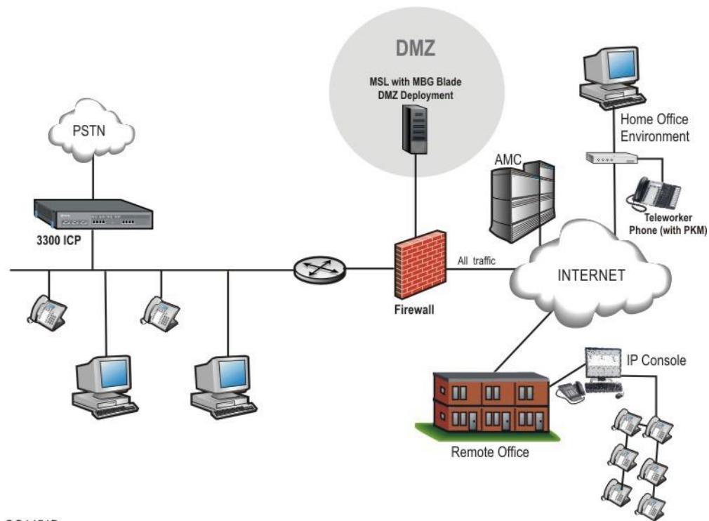
Figure 2. DMZ Configuration
