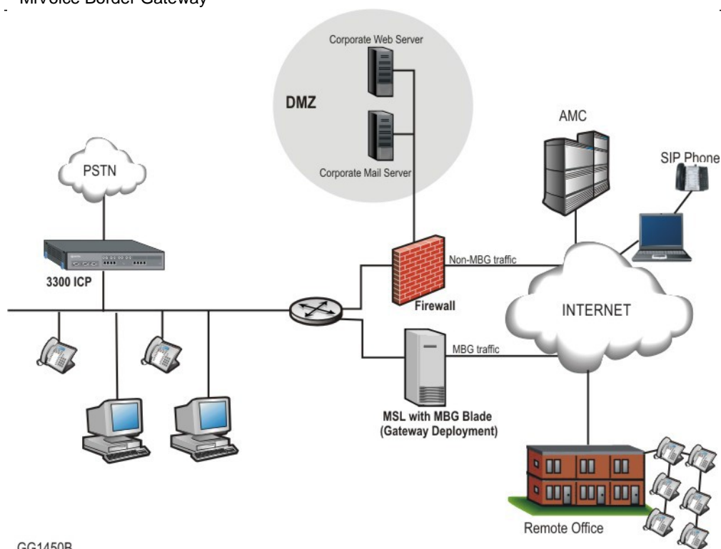
Figure 1. Server-Gateway Configuration
