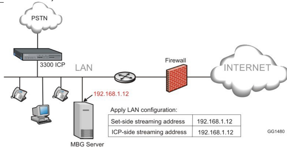
Figure 3. Server-only Configuration
