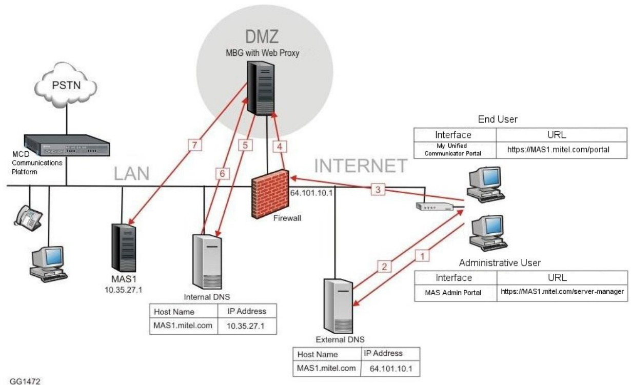
Figure 10. Basic Operation
