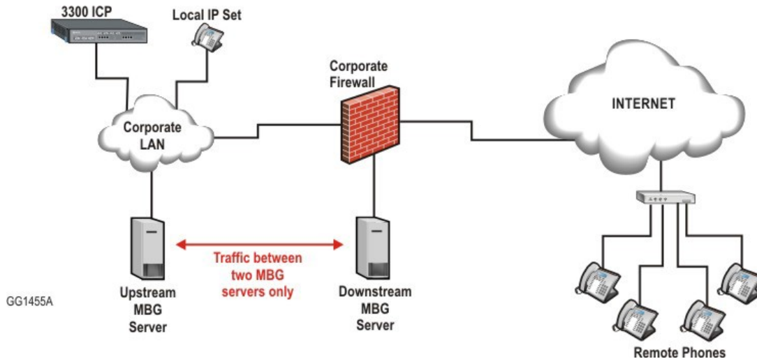
Figure 19. Daisy Chained Firewall Administrator
