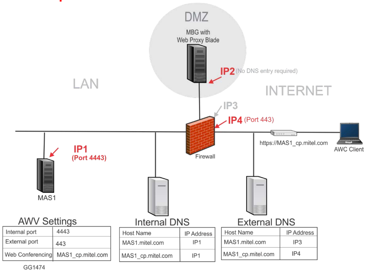
Figure 12. AWW Configuration with Additional Dedicated External IP Address
