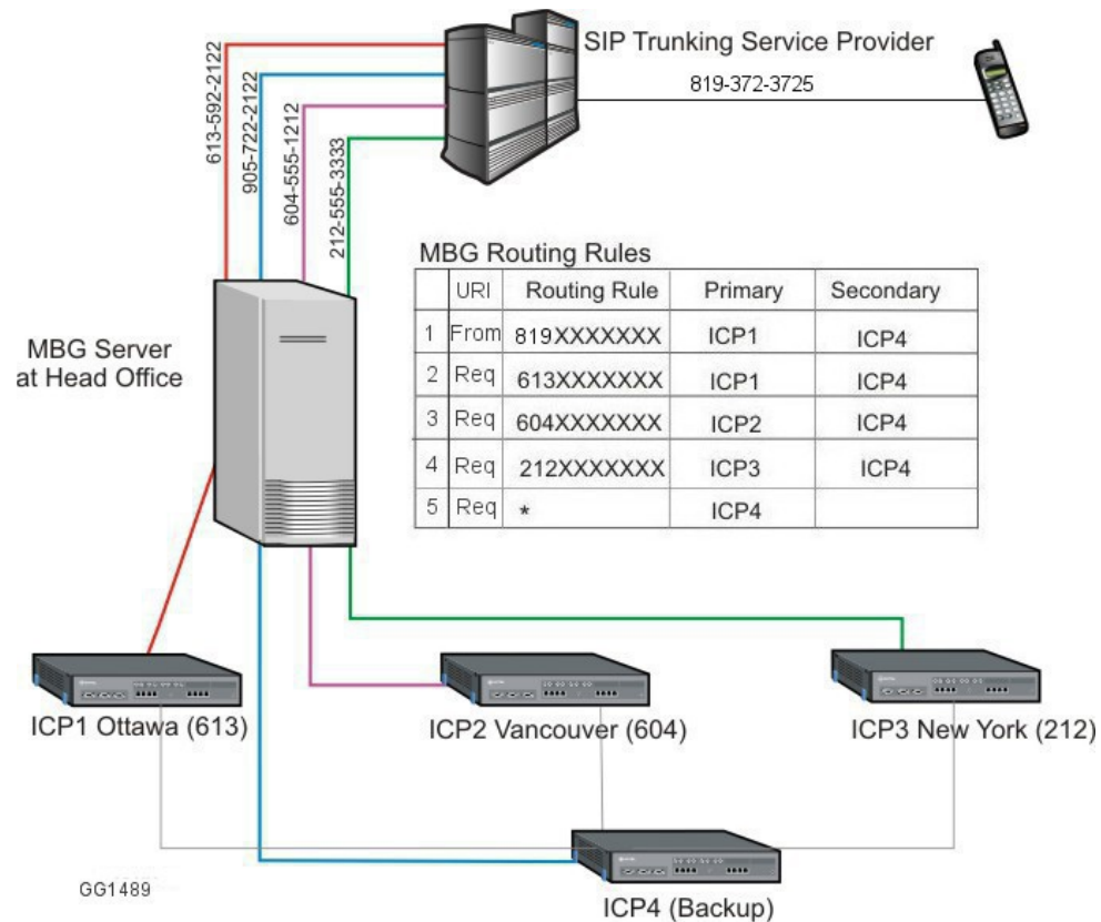
Figure 8. SIP Trunking Configuration Example with DID Routing Rules
