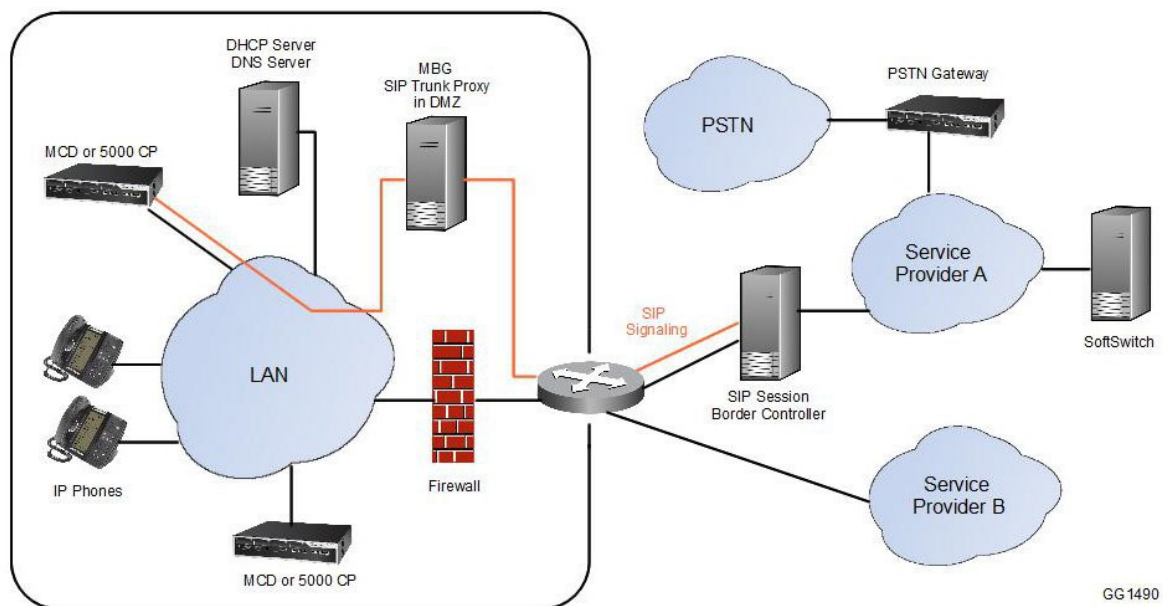
Figure 7. Configuration Example
