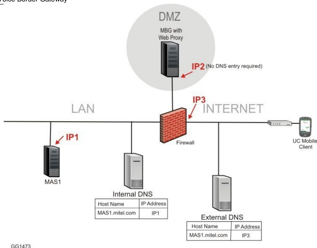
Figure 11. Basic DNS Configuration
