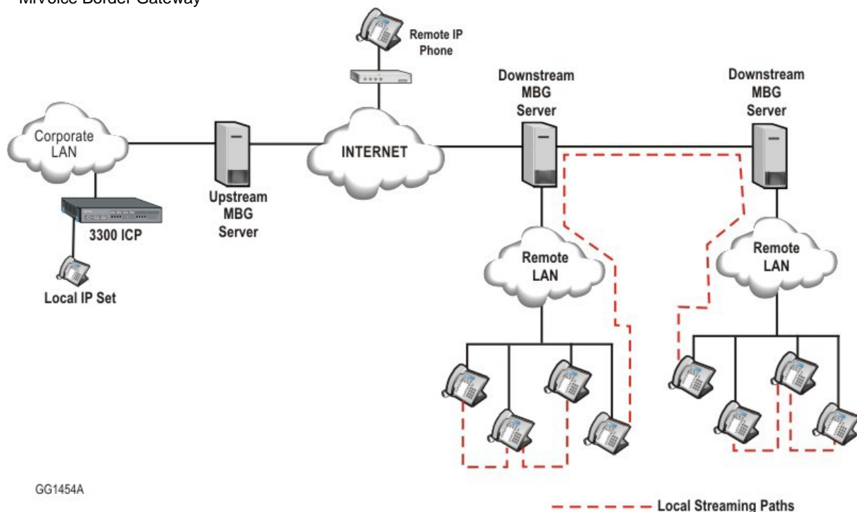
Figure 18. Daisy Chaining
