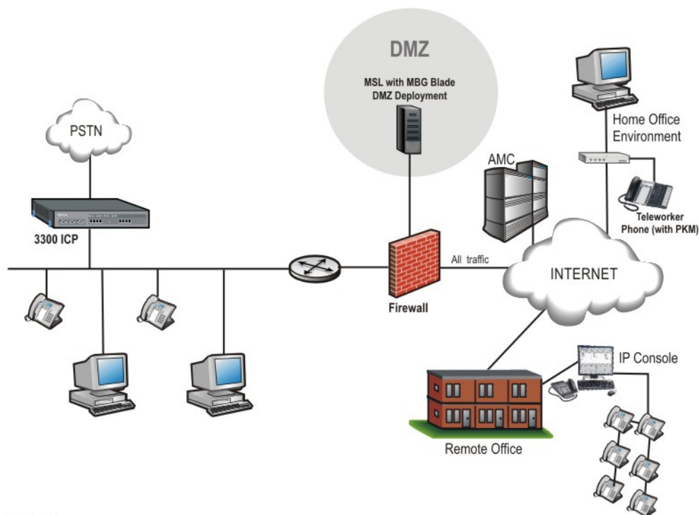
Figure 2. DMZ Configuration
