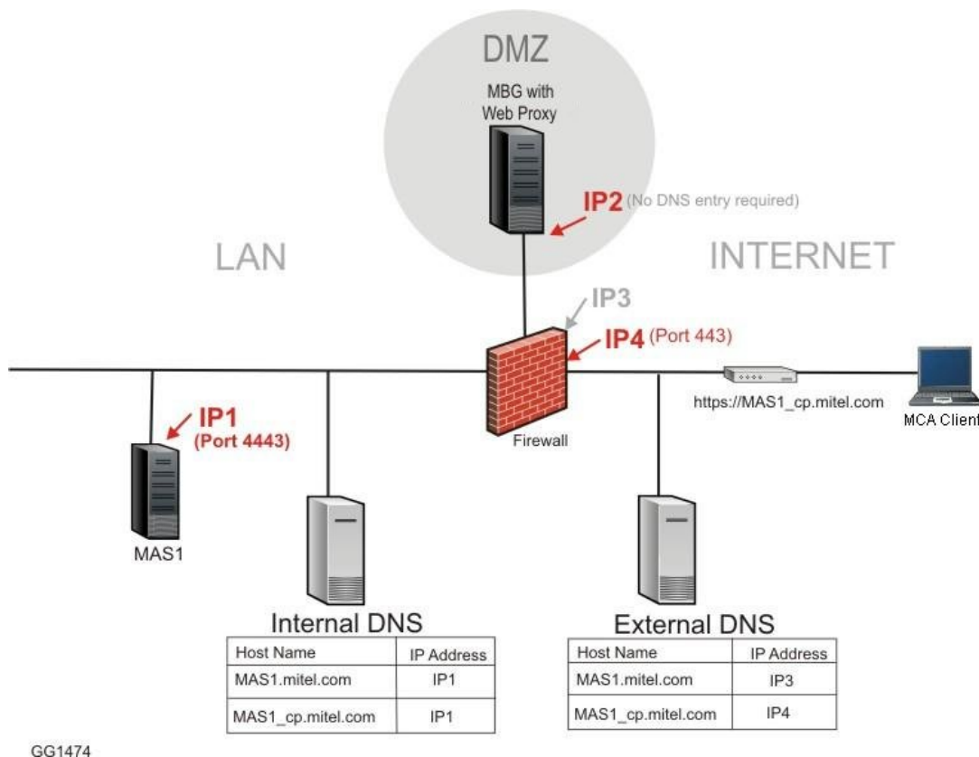
Figure 12. AWV Communications
