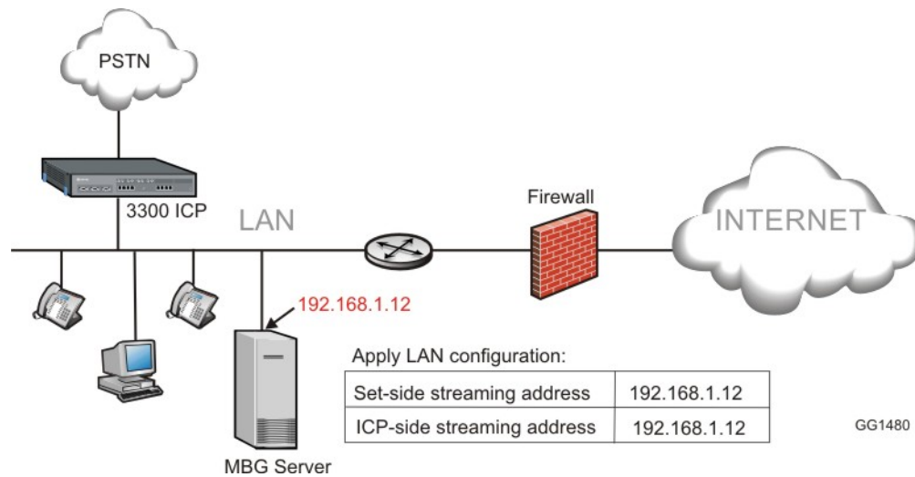
Figure 3. Server-only Configuration
