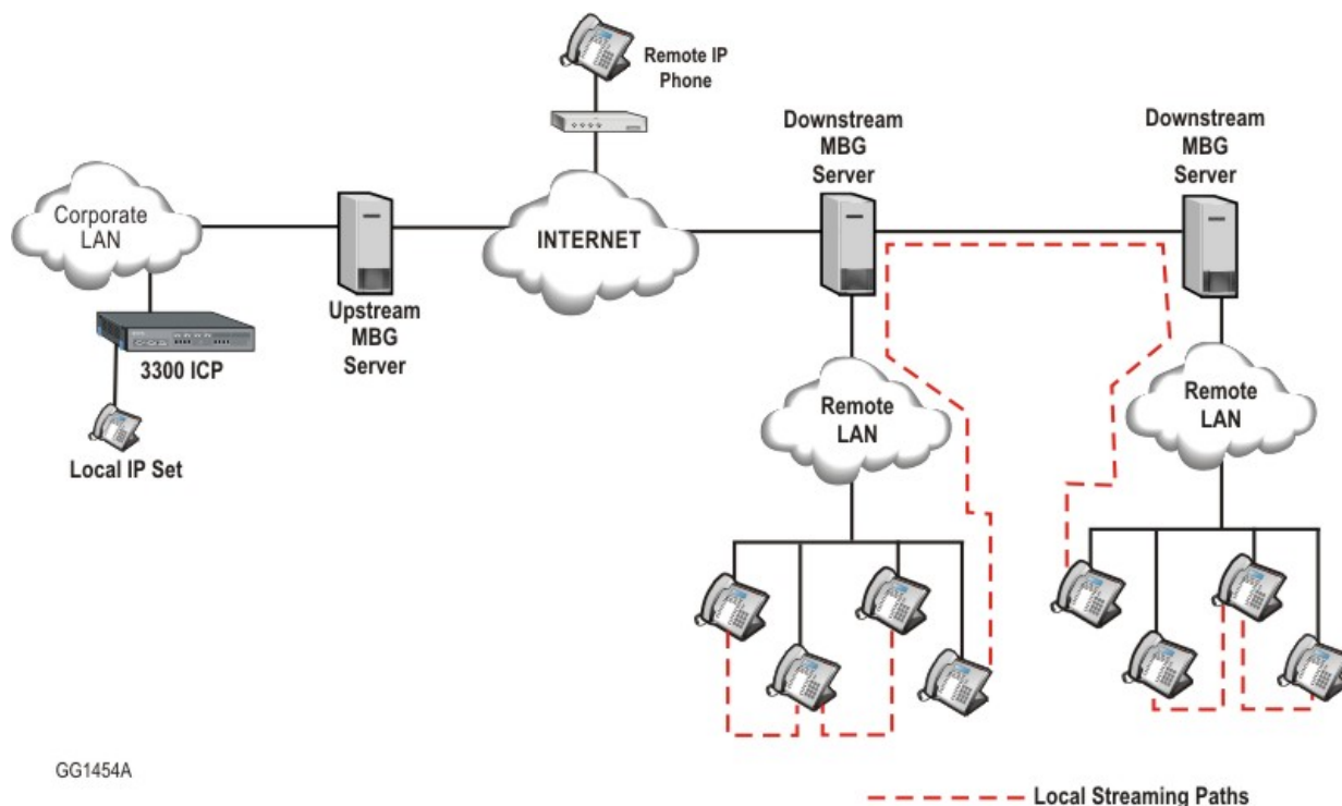
Figure 18. Daisy Chaining
