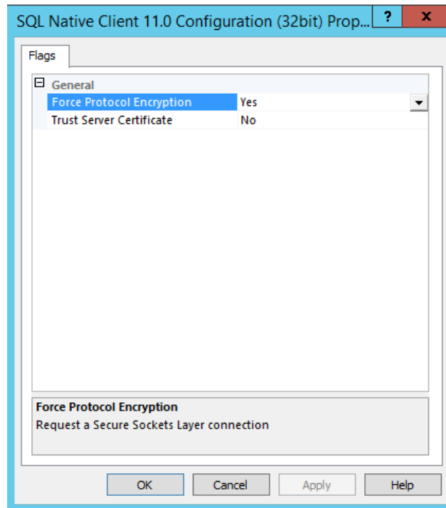
Figure 14: Native client protocol Force Protocol Encryption flag set to Yes
