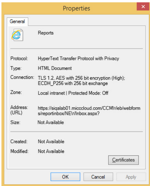
Figure 9: Page properties for CCMWeb showing TLS 1.2
