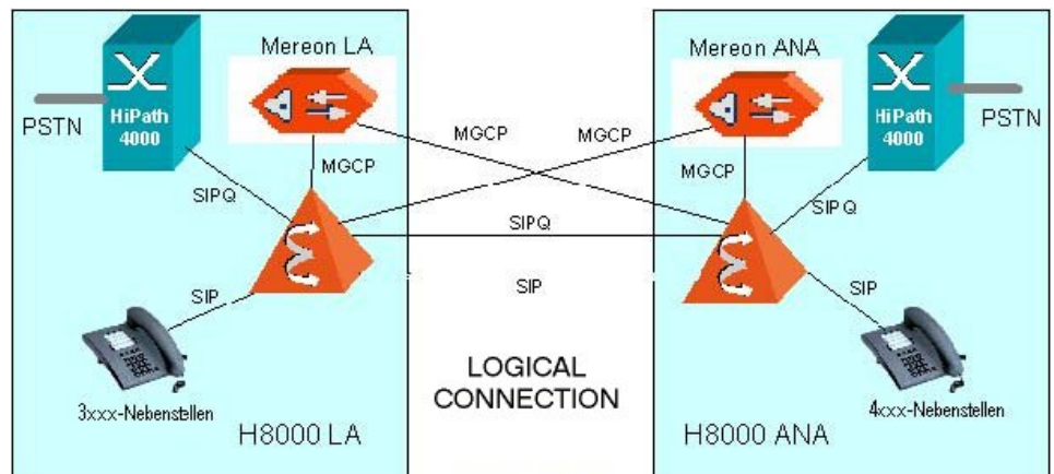
Figure 6: Two OpenScape Voice Systems in Simple SIP-Q Network -- Logical Connectivity
