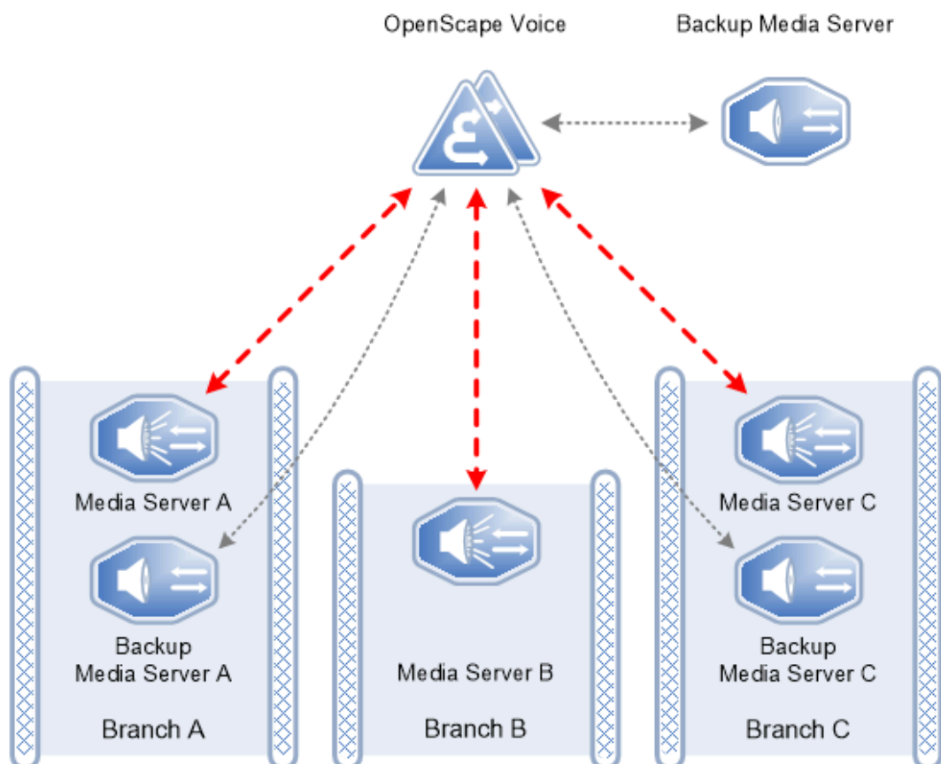
Figure 47: N+K redundancy – OpenScale Voice cluster nodes at the same branch
