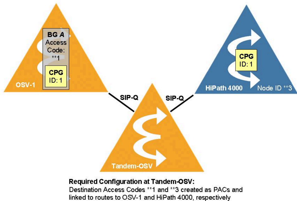
Figure 37: Network-wide CPG - Tandem Scenario (Example)
