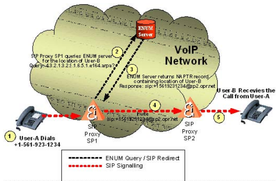
Figure 57: Simple SIP Call Flow with ENUM Query
