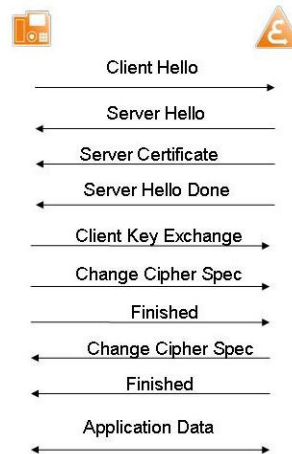
Figure 20 Sample TLS Connection Call Flow
