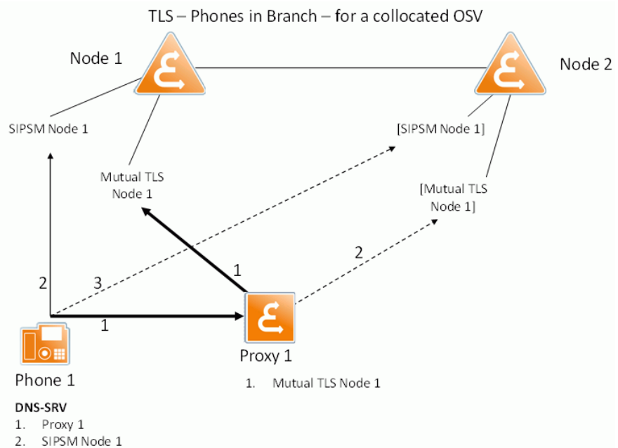
Figure 27 TLS-Phones in Branch for a Collocated System
