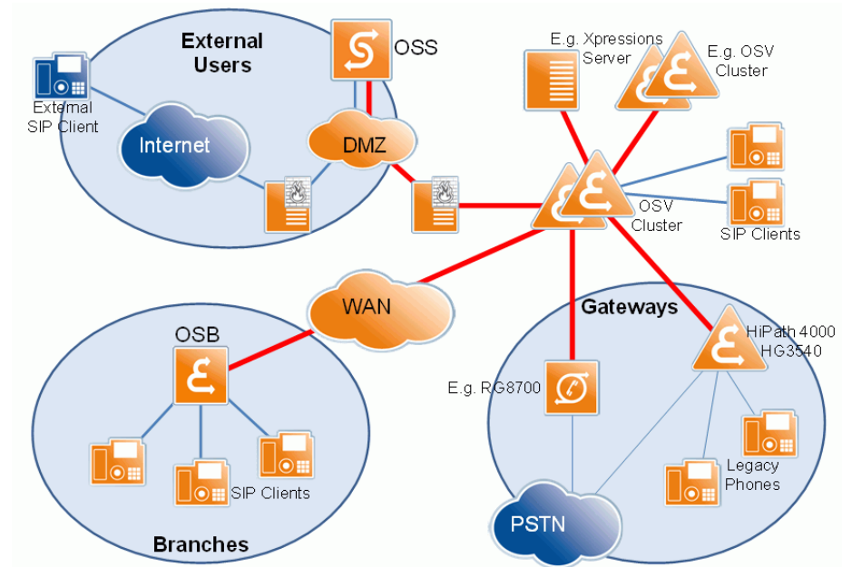
Figure 30 Deployment Recommendations
