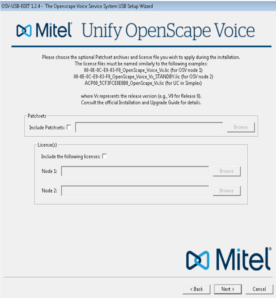
Figure 8 Patchset / License
