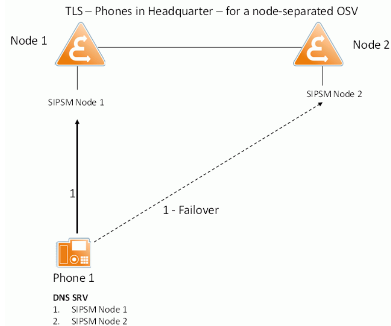
Figure 28 TLS - Phones in Headquarter for a Node Separated System
