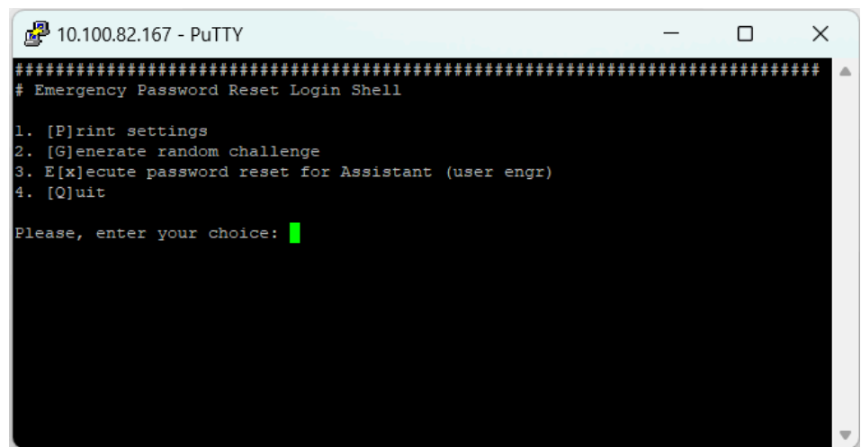
Figure 1: EPR login shell, initial menu
