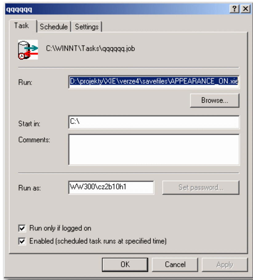
Figure 33: Scheduler API
