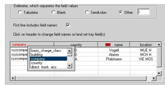
Figure 25: Editing Field Names in the Import Table
