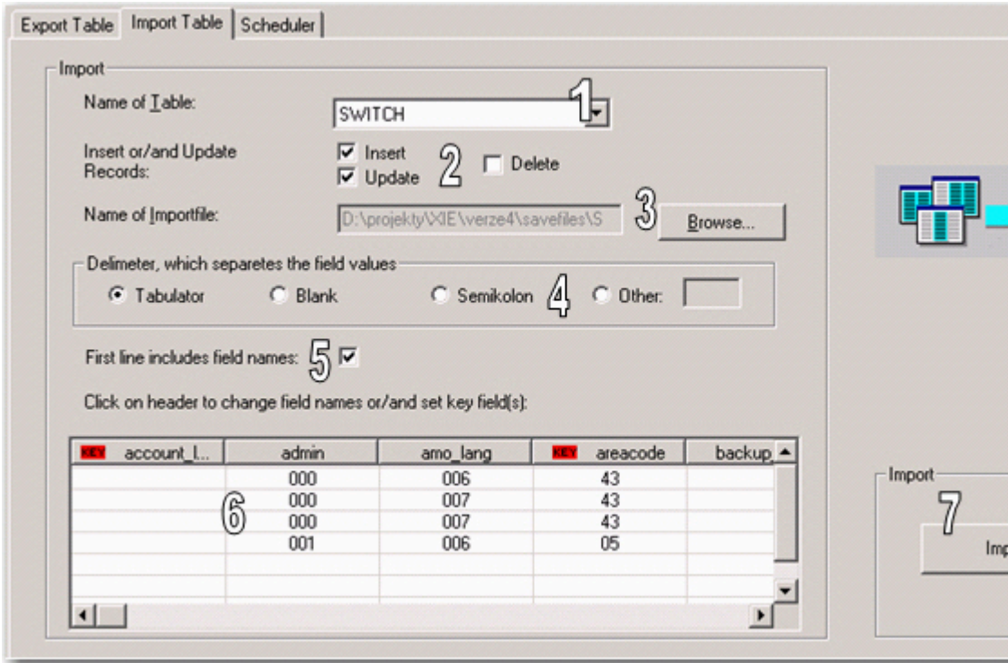
Figure 23: Import Table Property Page
