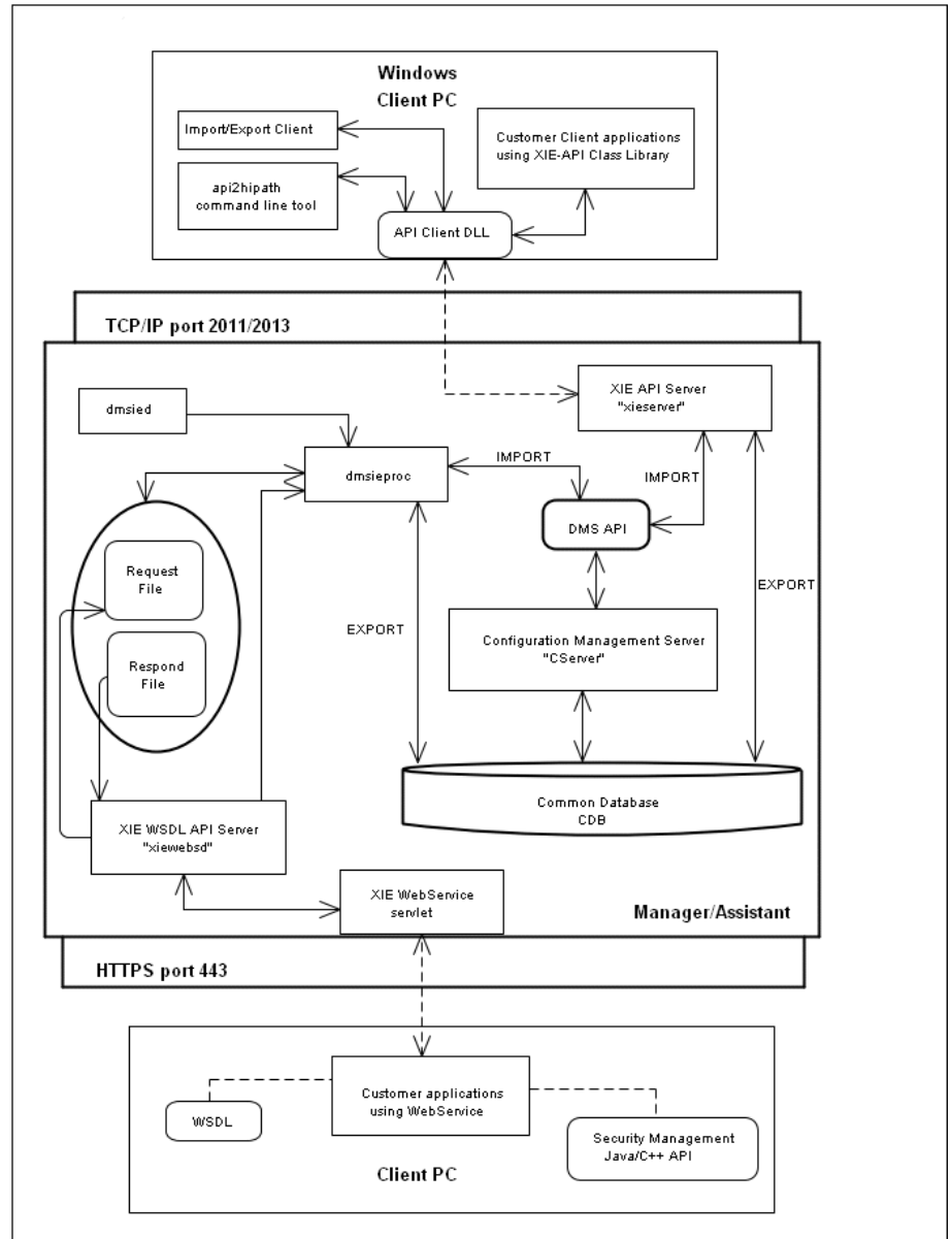
Figure 1: XIE-API Data Exchange
