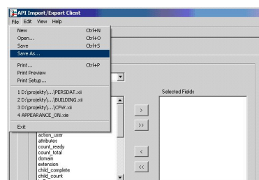
Figure 12: File Menu
