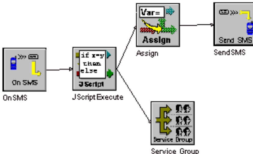
Figure 12: Incoming SMS
