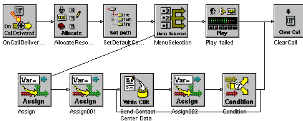
Figure 1: Logon Script
