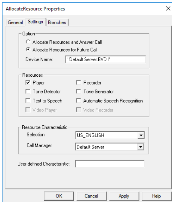
Figure 27: Allocate Resource for Future Call selected
