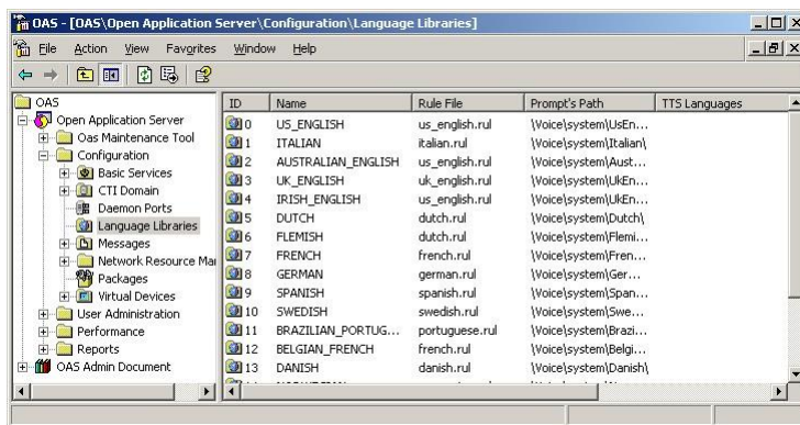
Figure 5 Language Libraries
