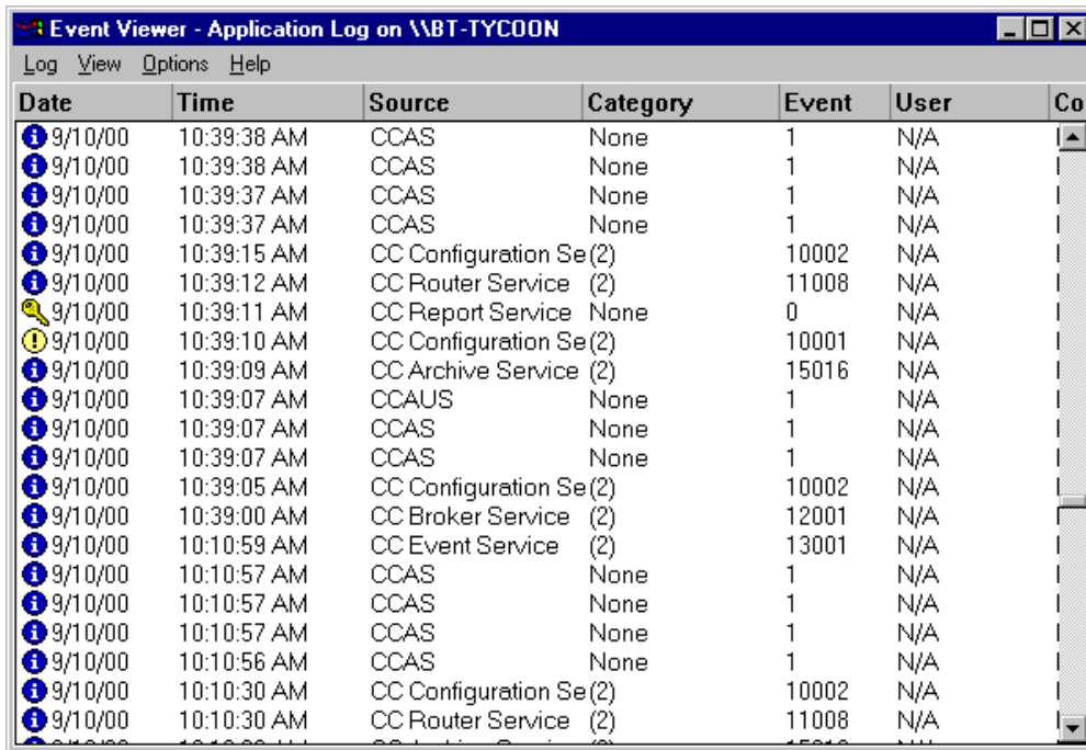
Figure 2: Application Log
