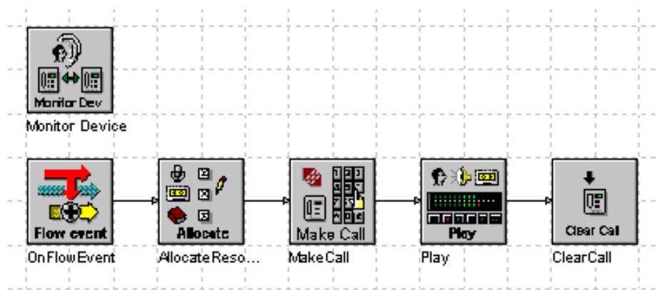
Figure 24: Event-Driven script
