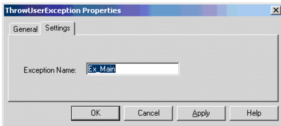
Figure 33: ThrowUserException
