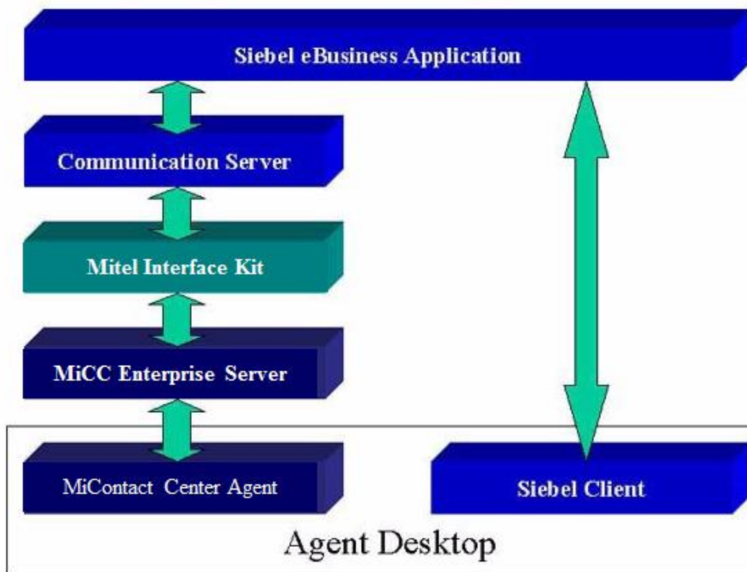
Figure 1: Commands and Event Flow
