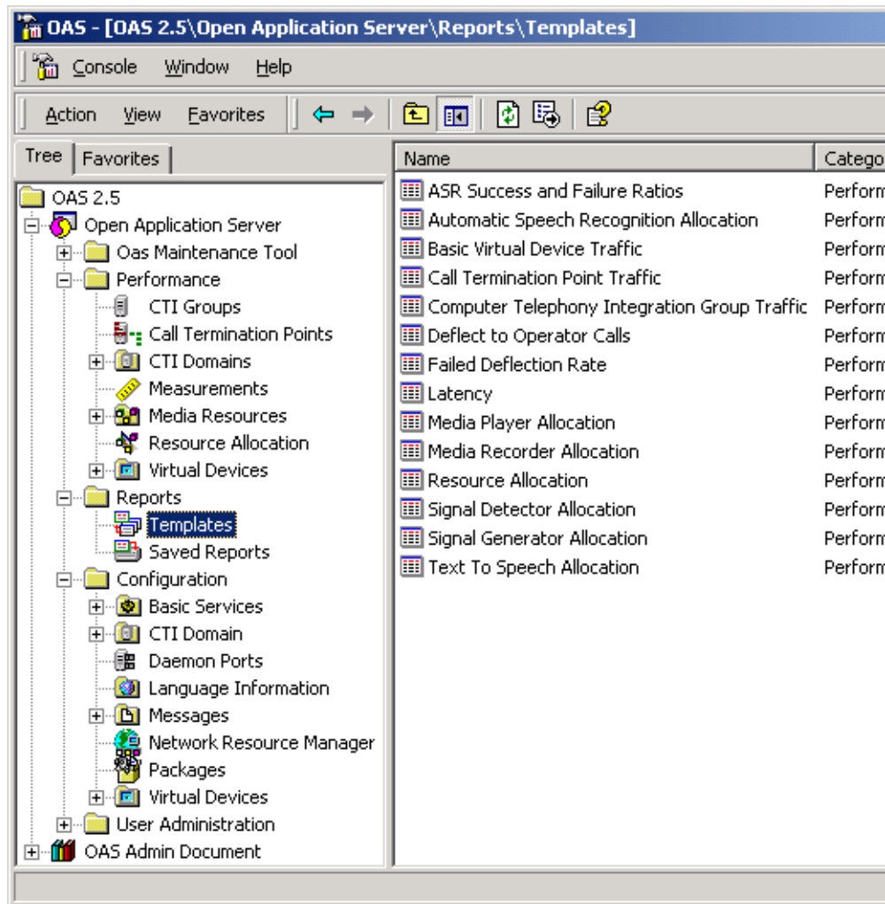
Figure 5: OAS Management Console screen
