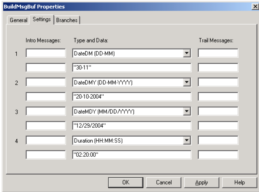
Figure 2 Build Message dialog box
