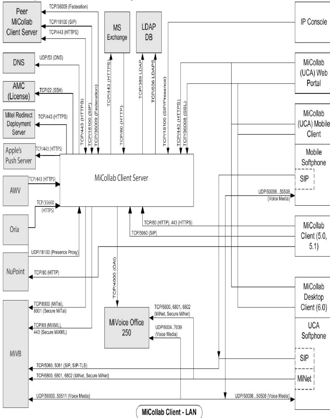
Figure 3.5: Ports needed by MiCollab Client Server on a Local Area Network (LAN)
