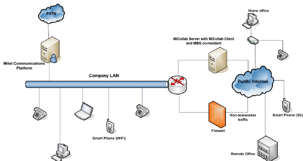
Figure 3.3: MiCollab Client Service in Server/Gateway Mode as part of MAS
