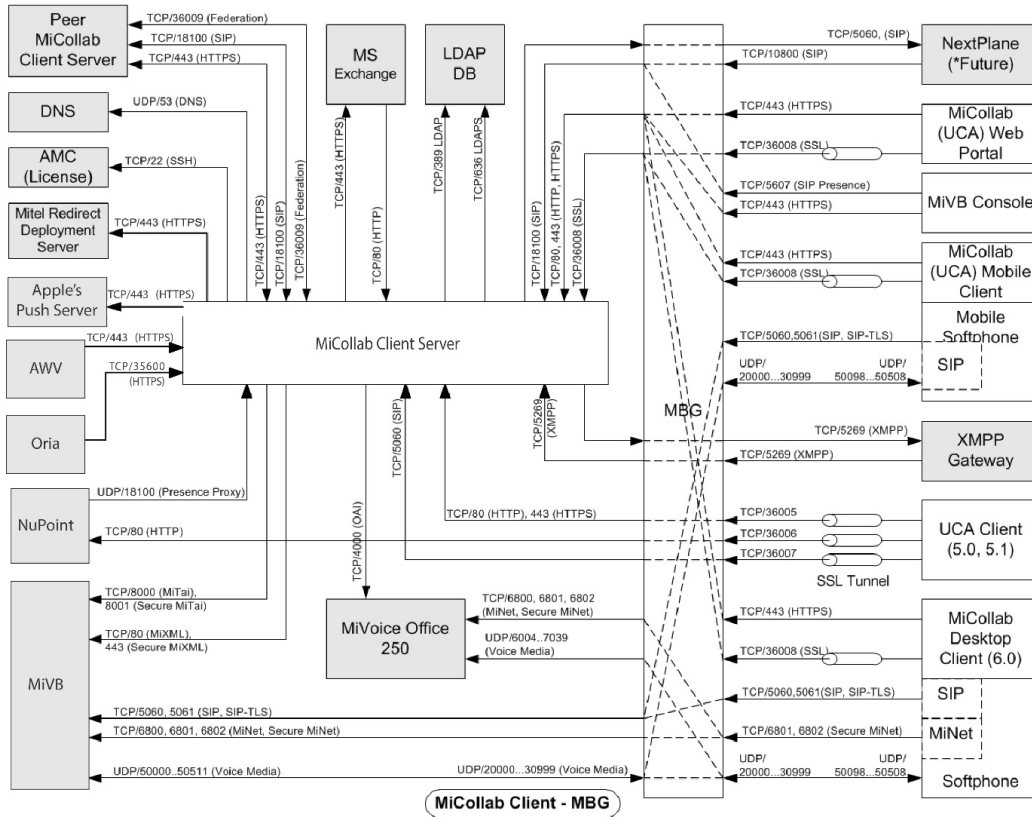
Figure 3.6: Ports needed by MiCollab Client Service on a Local Area Network (LAN) where the MiCollab Clients are required to connect via the MiVoice Border Gateway (MBG)
