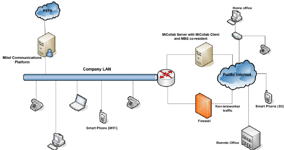
Figure 3.2: MiCollab Client Service in LAN with MBG and Web Proxy in network edge
