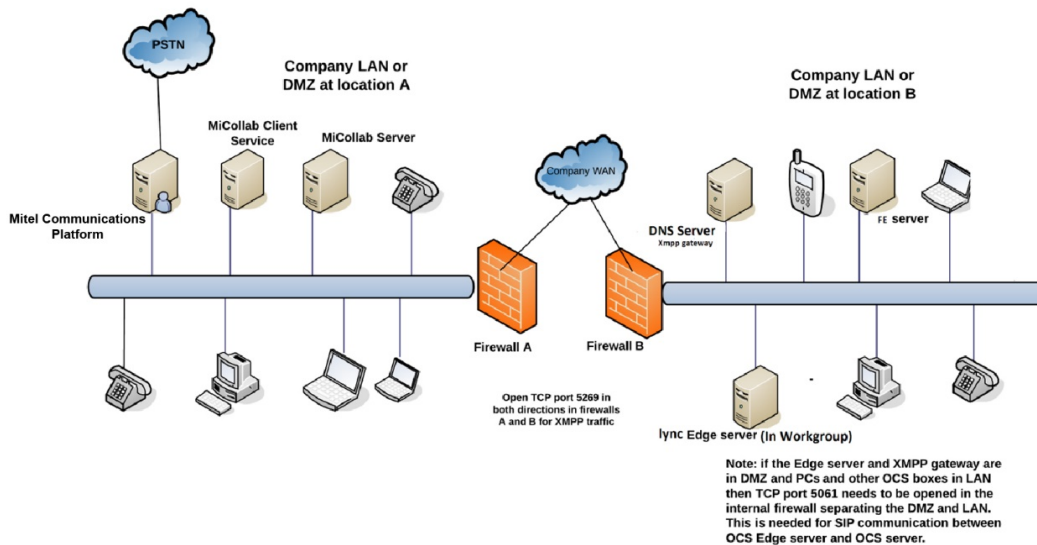
Figure 4.2: MiCollab Client Service Setup for IM and presence federation with OCS
