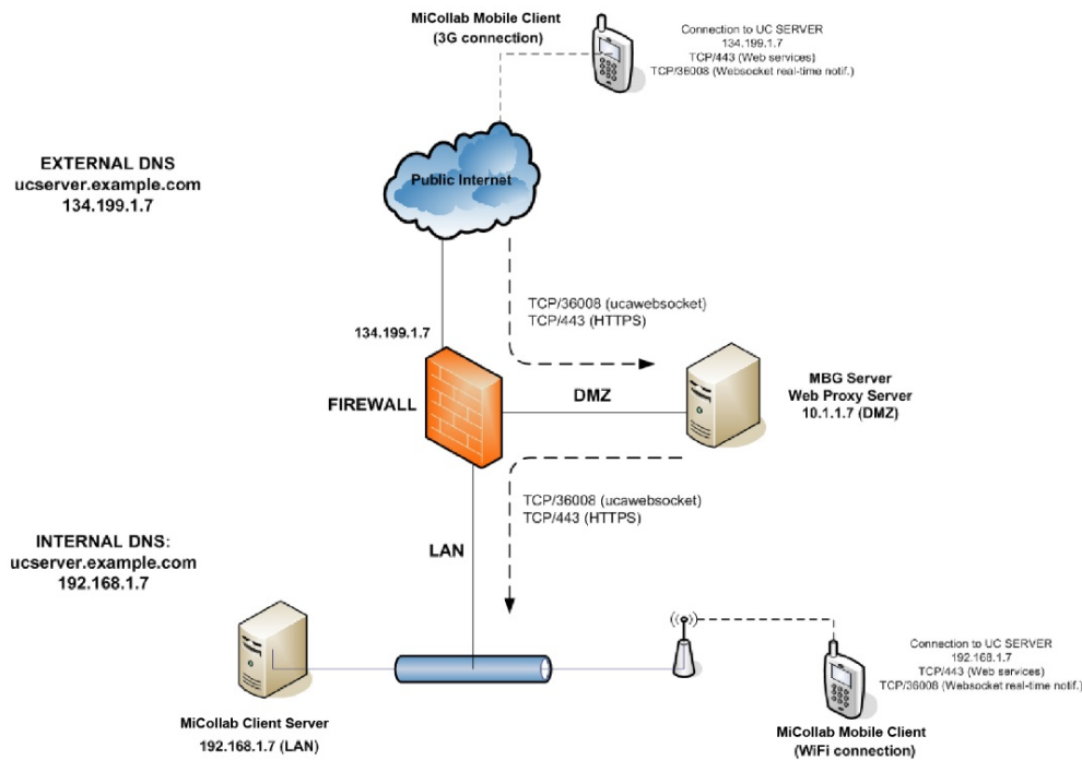
Figure 4.1: Configuring support for MiCollab Client Smart Devices when using an MBG in the DMZ
